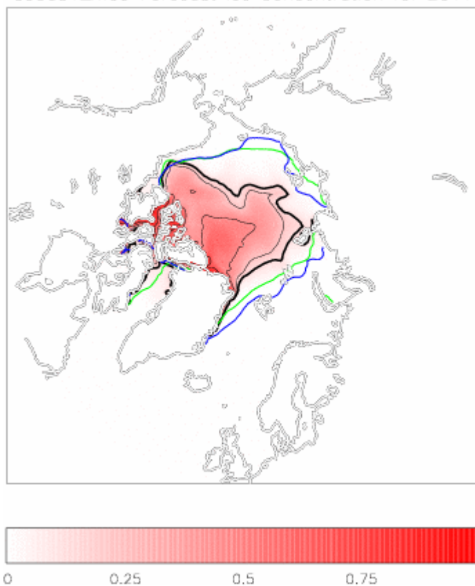
Figure 4. Forecast 2011 sea ice concentration. The thick black line is the forecast ice extent (ice concentration of 0.15) and the thinner black lines are contour intervals of 0.25. The green line is the model ice extent climatology during the hindcast period of 1996-2009, while the blue line is the observed climatological ice extent over the same period.
