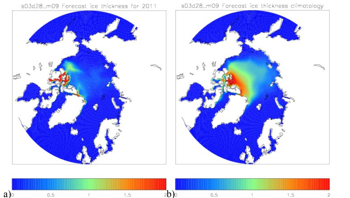
Figure 5. a) Forecast September 2011 ice thickness. b) Hindcast climatological ice thickness. Once again the colour shading saturates at 2m thick ice, but thicker ice does exist.
