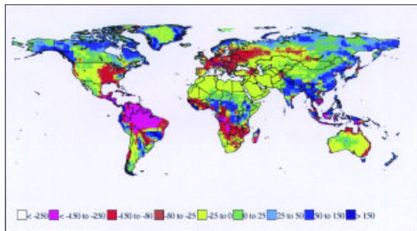
Estimated change in 30-year mean annual runoff (millimetres per year) by the 2050s, compared with the baseline period.
