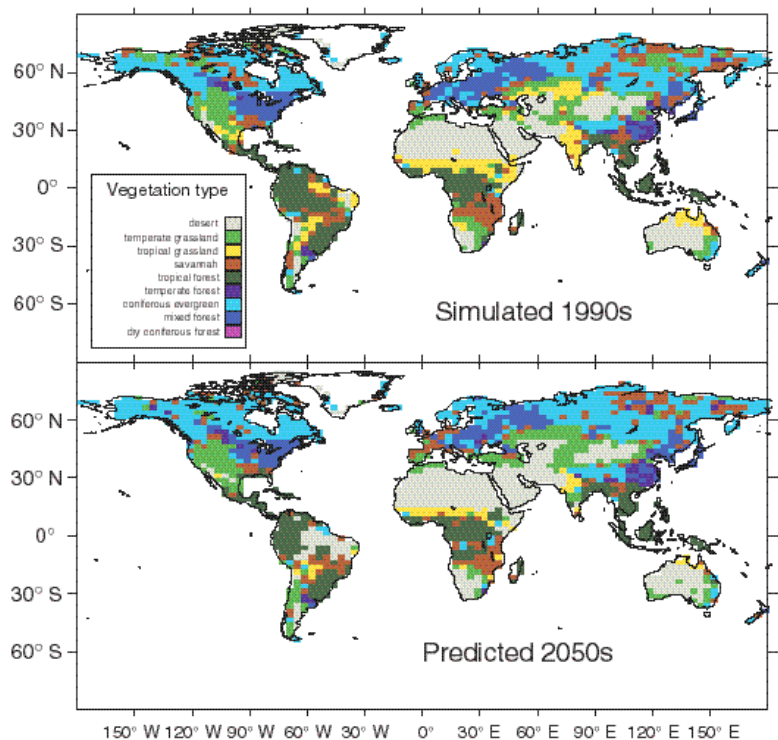
Global distribution of vegetation types predicted by the ITE ecosystem model for the present day and for the 2050s.
