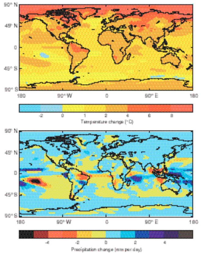
The patterns of change in northern winter temperature (top) and precipitation (bottom) for the 2050s, compared to the present day, when the climate model is driven with IPCC 'business-as-usual' changes in greenhouse gases only.
