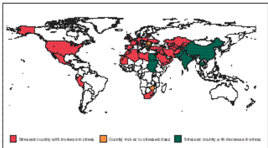
Change in water stress, due to climate change, in countries using more than 20% of their water resources.
