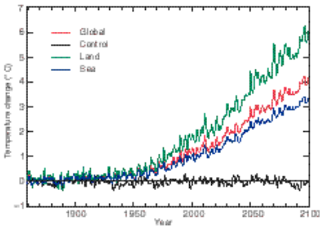
Changes in land, sea and global mean surface temperature from the new Hadley Centre model driven with changes in greenhouse gas concentrations (without sulphate aerosols): observed to 1995 and IPCC 'business-as-usual' to 2100. The black line shows the low climate drift of the unperturbed model.
