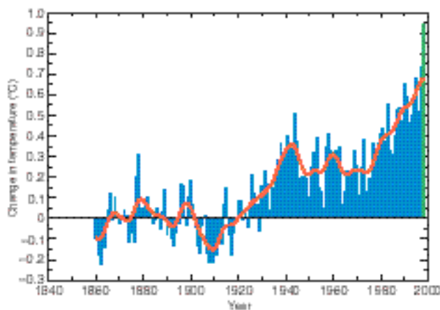
Changes in the global annual mean surface temperature, relative to that at the end of the last century, are shown by blue bars, with a smoothed curve in red. The value for 1998, shown in green, includes observations up to the end of September.
