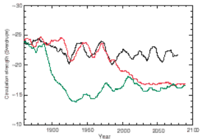
The strength of the Atlantic circulation is seen to decrease substantially as greenhouse gas concentrations rise at 2% per year to four times the pre-industrial value (green). The black line shows the unperturbed circulation, and the red line the change when greenhouse gases follow the IPCC 'business-as-usual' emissions scenario.
