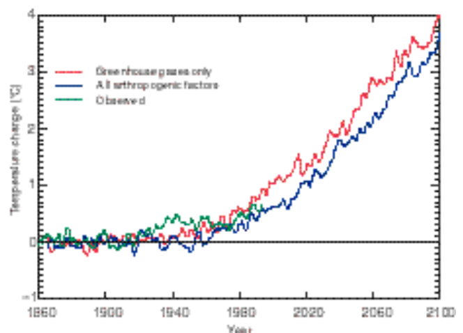
The global mean surface temperature change when the model includes the effect of greenhouse gases (red), and also including the direct and indirect effects of sulphate aerosols (blue). Observations are shown in green.
