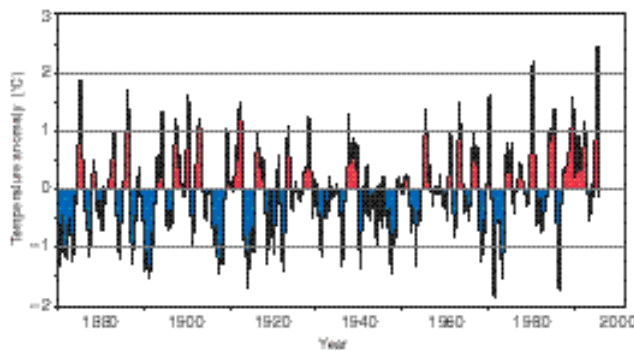
Changes in sea-surface temperature 1871–1998, relative to the 1961–90 average, for the eastern tropical Pacific off Peru.
