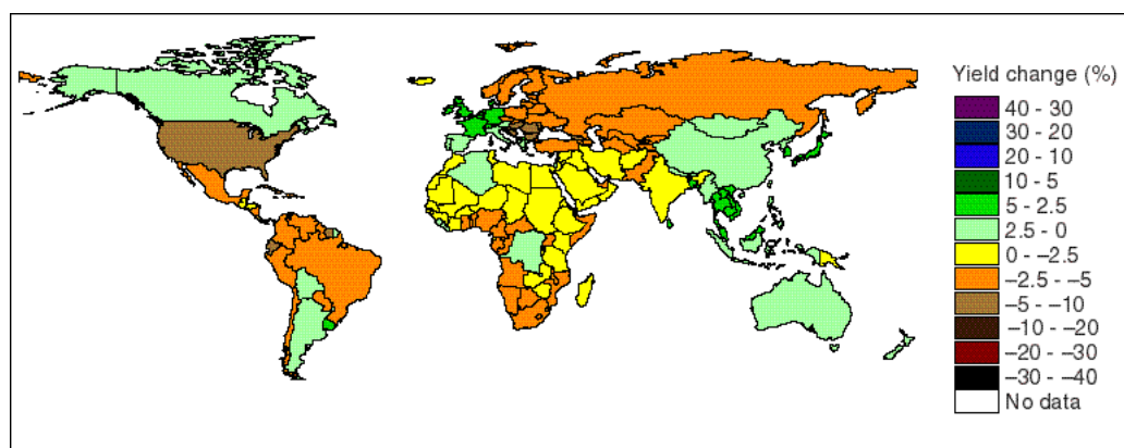
Potential change in yields of cereals (wheat, maize, rice) for the 2050s, including effects of CO 2 .
