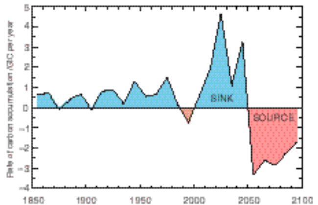
Predicted changes in the rate of increase in the carbon store on land, showing when the land is a source or sink of carbon.
