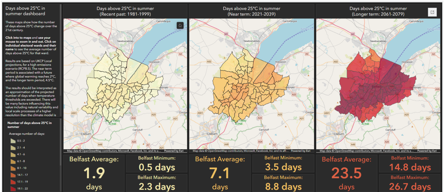
ArcGIS Dashboards
