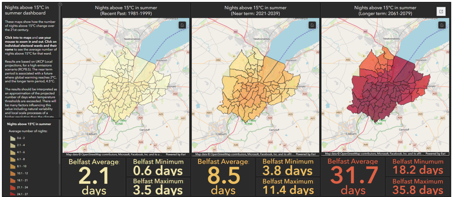
ArcGIS Dashboards
