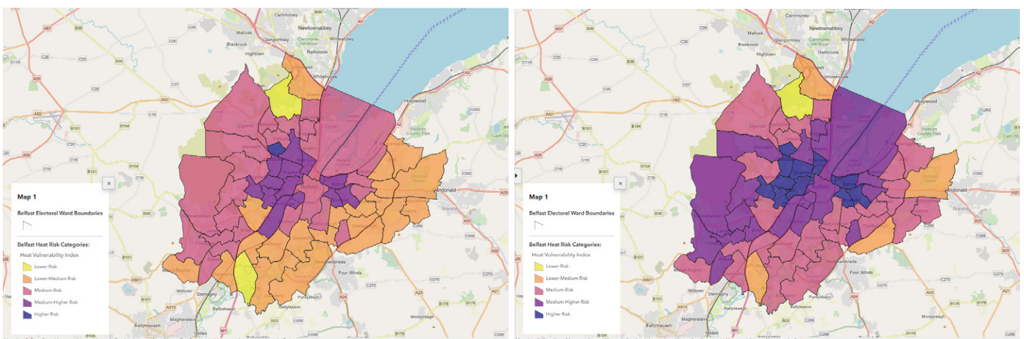
The map on the left shows heat risk for 2021-2039 (~2°C world) time period, the map on the right is for 2061-2079 (~4.5°C world).
