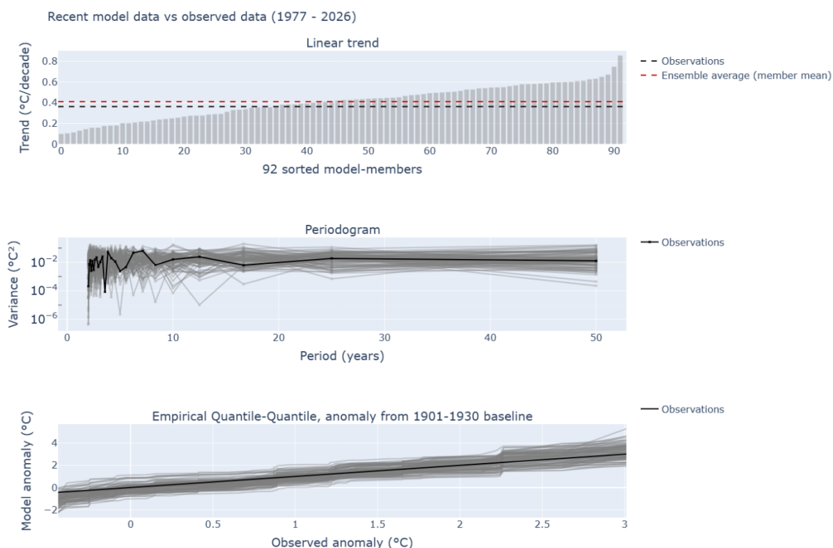
Figure 5: Evaluation of CMIP6 multi-model ensemble used in the attribution analysis, for recent experiments (combined historical and ssp245 experiments), evaluated over 1977 – 2026 by comparison with observational HadUK-Grid data. Top panel: temperature trends over the evaluation period. Middle panel: power spectra estimates (periodogram) from the HadUK-Grid data and recent simulations. Bottom panel: quantile-quantile plot for each of the recent simulations.
