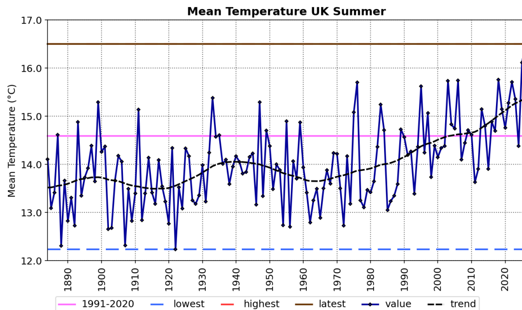
Figure 2: UK summer mean temperature from 1884 to 2026. The smoothed trend is shown as a black dashed curve. The 1991-2020 summer average is shown as a pink line.
