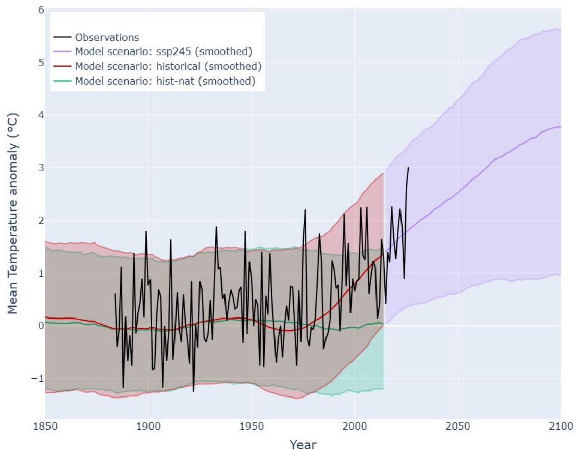
Figure 3: Time series of the UK summer mean temperature anomaly (w.r.t. 1901 – 1930). Observational data from HadUK-Grid (black). Simulations from the CMIP6 historical (red), ssp245 (purple) and hist-nat (green) experiments. Simulation data is represented as median values and filled 5 th – 95 th percentile ranges explored by members of the multi-model ensemble. Simulation data is smoothed with a rolling window of 20 years, with historical and ssp245 combined into one continuous series. Observed data runs from 1884 – 2026.
