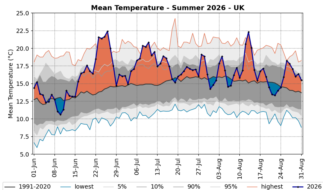
Figure 1: UK daily mean temperature for summer 2026. Periods of above average temperature are highlighted orange, and periods below average are blue. The 1991-2020 average temperature is shown in black. The (light) grey shaded regions show the (5%-95%) 10%-90% of all summers, and the thin orange and blue outer lines show the daily record temperatures. The thick blue line shows 2026 daily mean temperatures.
