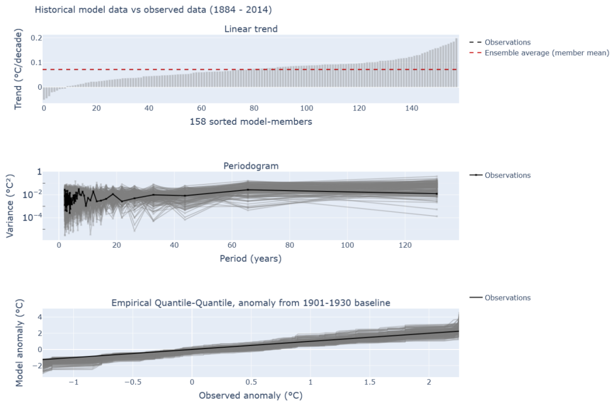
Figure 4: Evaluation of CMIP6 multi-model ensemble used in the attribution analysis, for the historical experiment, evaluated over 1884 – 2014 by comparison with observational HadUK-Grid data. Top panel: temperature trends over the evaluation period. Middle panel: power spectra estimates (periodogram) from the HadUK-Grid data and historical simulations. Bottom panel: quantile-quantile plot for each of the historical simulations.
