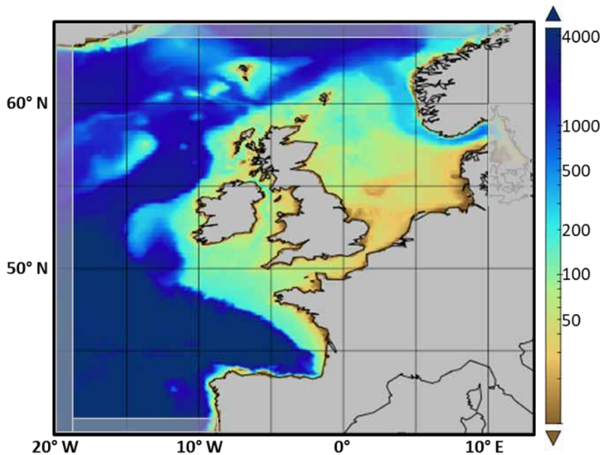
Bathymetry of the AMM7 model domain. The grey translucent areas show where the model output is masked.
