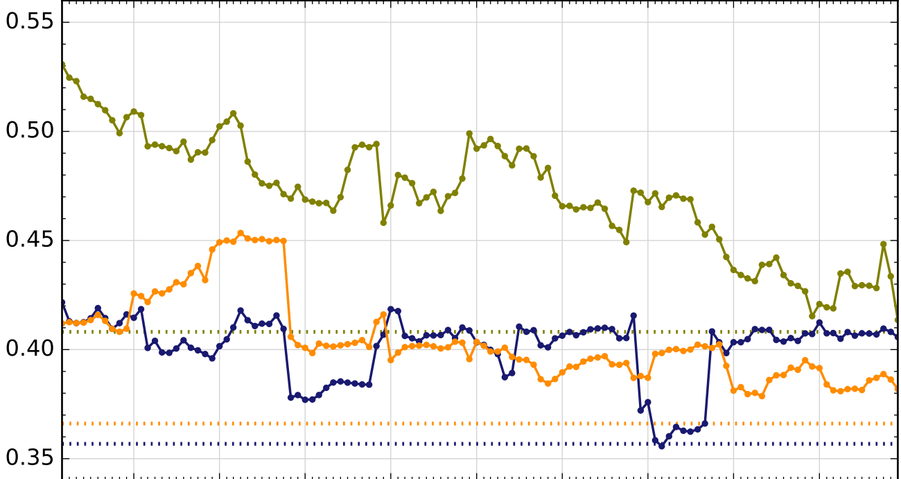
Visibility
