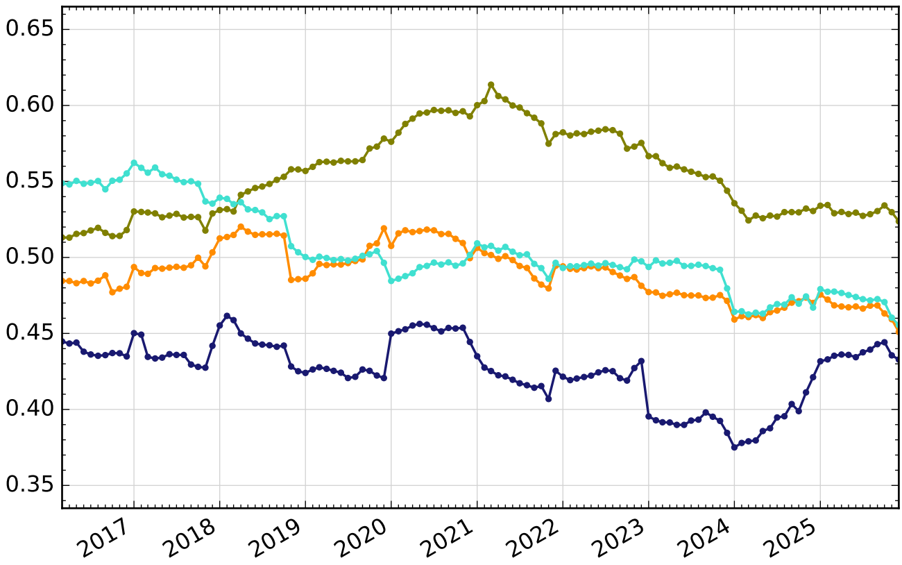
Cloud Base
