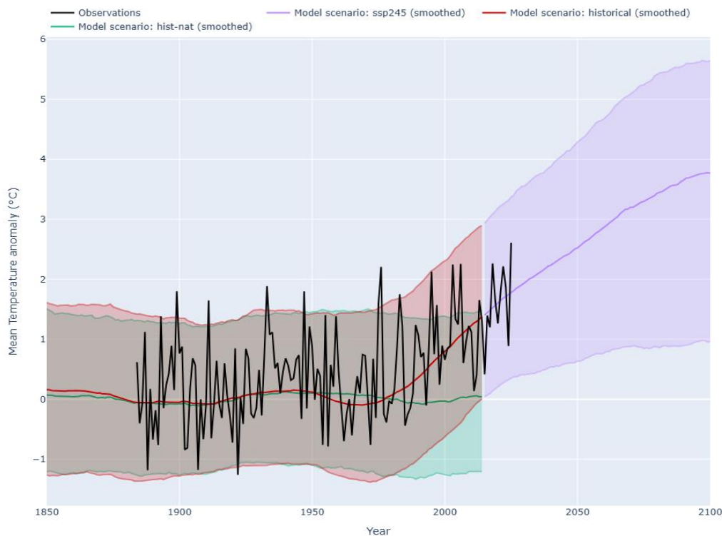
Figure 3: Time series of the UK summer mean temperature anomaly (w.r.t. 1901 – 1930). Observational data from HadUK-Grid (black). Simulations from the CMIP6 historical (red), ssp245 (purple) and hist-nat (green) experiments. Simulation data is represented as median values and filled 5 th – 95 th percentile ranges explored by members of the multi-model ensemble. Simulation data is smoothed with a rolling window of 20 years, with historical and ssp245 combined into one continuous series. Observed data runs from 1884 – 2025.
