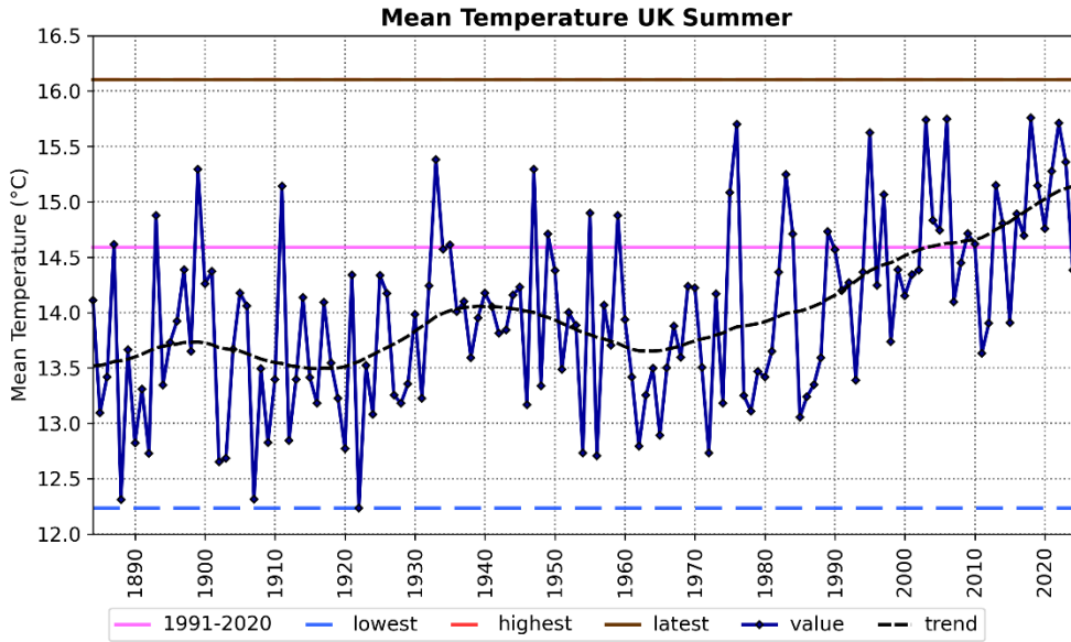
Figure 2: UK summer mean temperature from 1884 to 2025. The smoothed trend is shown as a black dashed curve. The 1991-2020 summer average is shown as a pink line.
