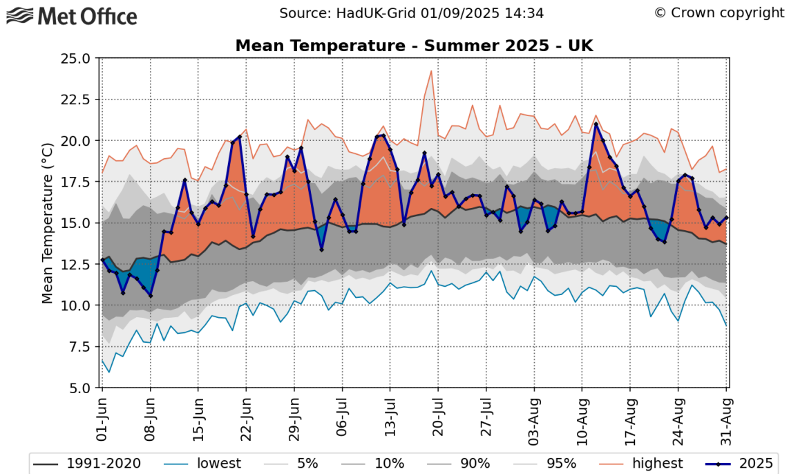
Figure 1: UK daily mean temperature for summer 2025. Periods of above average temperature are highlighted orange, and periods below average are blue. The 1991-2020 average temperature is shown in black. The (light) grey shaded regions show the (5%-95%) 10%-90% of all summers, and the thin orange and blue outer lines show the daily record temperatures.
