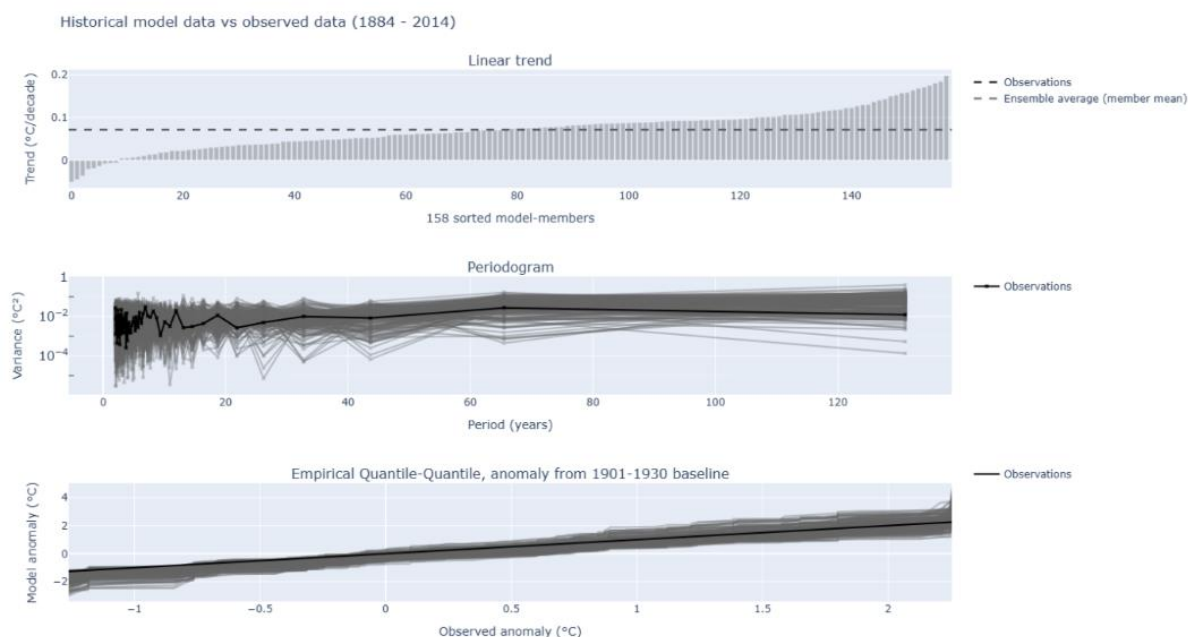
Figure 4: Evaluation of CMIP6 multi-model ensemble used in the attribution analysis, for the historical experiment, evaluated over 1884 – 2014 by comparison with observational HadUK-Grid data. Top panel: temperature trends over the evaluation period. Middle panel: power spectra estimates (periodogram) from the HadUK-Grid data and historical simulations. Bottom panel: quantile-quantile plot for each of the historical simulations.
