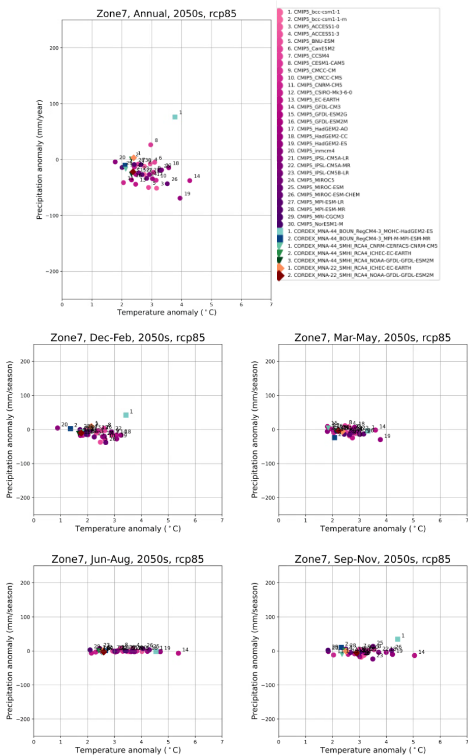
Figure B14: Projected change in average annual (top panel) and seasonal (bottom panels) precipitation and temperature in Zone 7. Each dot shows the difference between the average projected values in the 2050s and the average values in the current climate, for each climate model. Individual models are identified by the icon and number in the legend.
