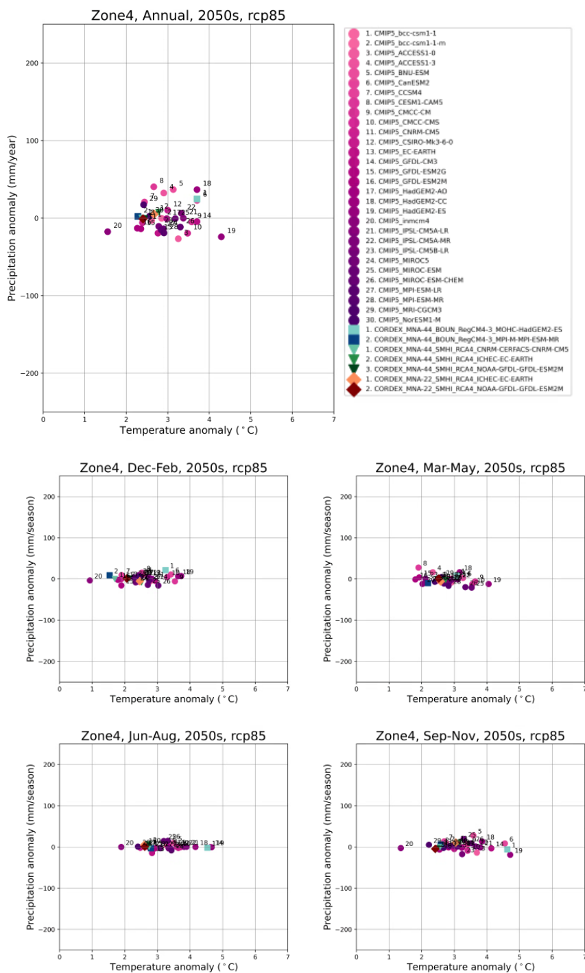
Figure B8: Projected change in average annual (top panel) and seasonal (bottom panels) precipitation and temperature in Zone 4. Each dot shows the difference between the average projected values in the 2050s and the average values in the current climate, for each climate model. Individual models are identified by the icon and number in the legend.
