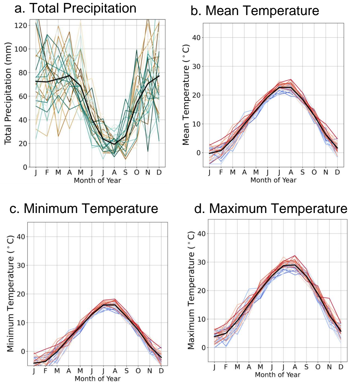
Figure B11: Observations of total monthly precipitation (a) and average daily mean (b), minimum (c) and maximum (d) temperature over the baseline period (1981-2010) for Zone 6. Each line is one individual year. Colours show the ordering of years from brown-blue (total precipitation) and blue-red (mean temperature) – this highlights the presence, or lack of, a trend over the baseline period. The bold black line indicates the average of the 30-year period.
