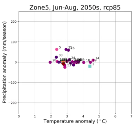
Figure B10: Projected change in average annual (top panel) and seasonal (bottom panels) precipitation and temperature in Zone 5. Each dot shows the difference between the average projected values in the 2050s and the average values in the current climate, for each climate model. Individual models are identified by the icon and number in the legend.
