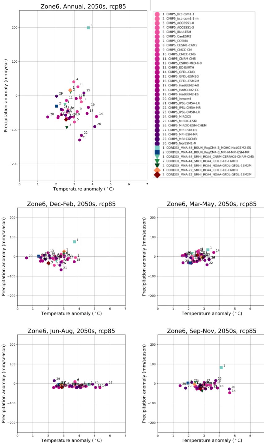
Figure B12: Projected change in average annual (top panel) and seasonal (bottom panels) precipitation and temperature in Zone 6. Each dot shows the difference between the average projected values in the 2050s and the average values in the current climate, for each climate model. Individual models are identified by the icon and number in the legend.
