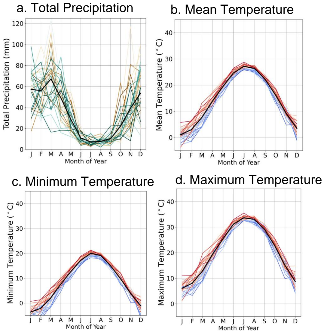
Figure B5: Observations of total monthly precipitation (a) and average daily mean (b), minimum (c) and maximum (d) temperature over the baseline period (1981-2010) for Zone 3. Each line is one individual year. Colours show the ordering of years from brown-blue (total precipitation) and blue-red (mean temperature) – this highlights the presence, or lack of, a trend over the baseline period. The bold black line indicates the average of the 30-year period.
