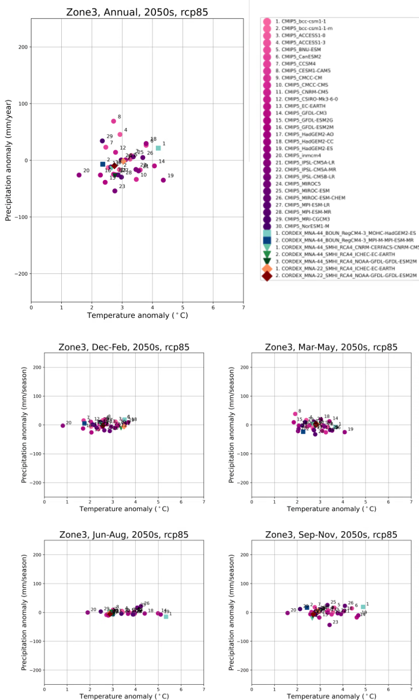
Figure B6: Projected change in average annual (top panel) and seasonal (bottom panels) precipitation and temperature in Zone 3. Each dot shows the difference between the average projected values in the 2050s and the average values in the current climate, for each climate model. Individual models are identified by the icon and number in the legend.
