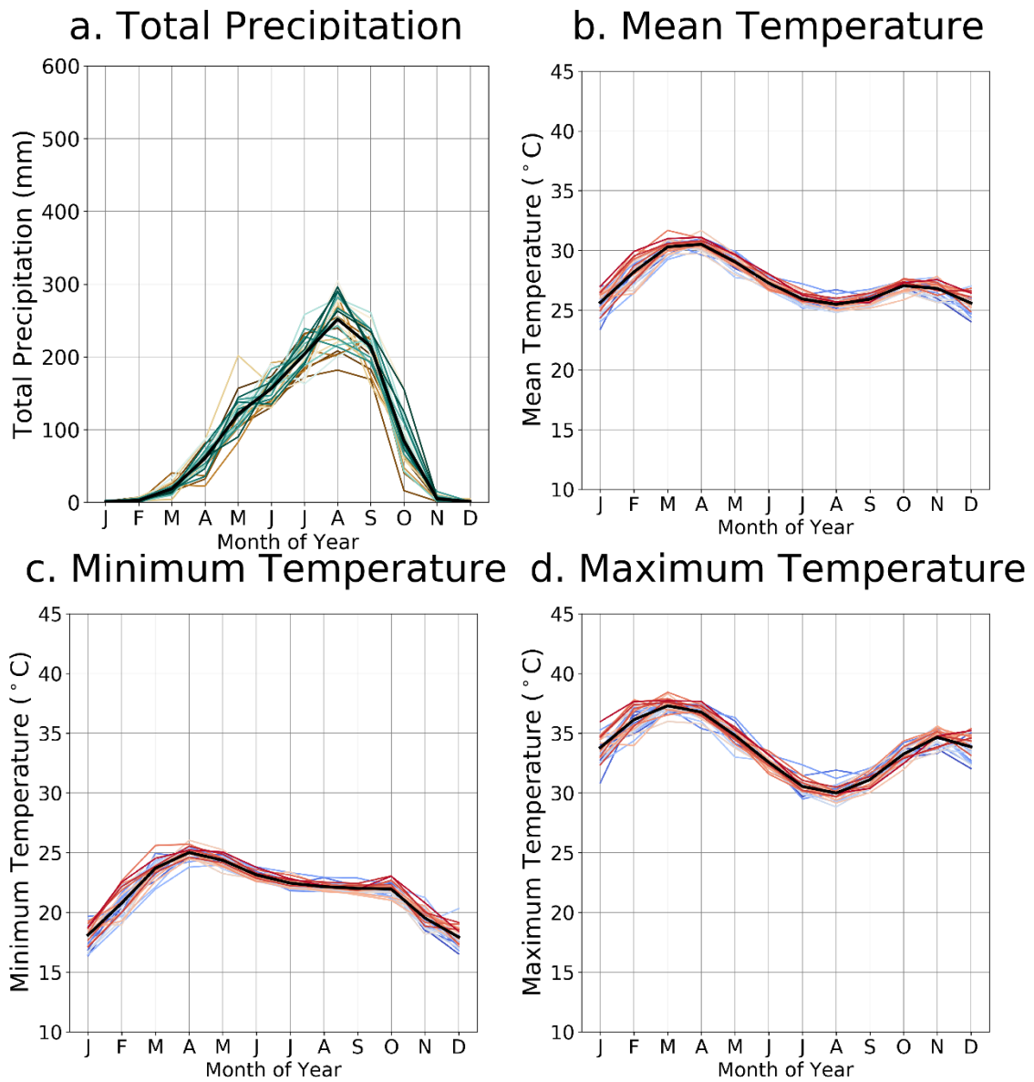
Figure B7: Observations for Zone 4 of total monthly precipitation (a) and average daily mean (b), minimum (c) and maximum (d) temperature over the baseline period (1981-2010). Precipitation data from CHIRPS (Climate Hazards group Infrared Precipitation with Stations) and temperature data from WFDEI-CRU (WATCH Forcing Data methodology applied to ERA-Interim data). Each line is one individual year. Colours show the ordering of years from brown to blue (total precipitation) and blue to red (mean temperature) – this highlights the presence, or lack of, a trend over the baseline period. The bold black line indicates the average of the 30-year period.
