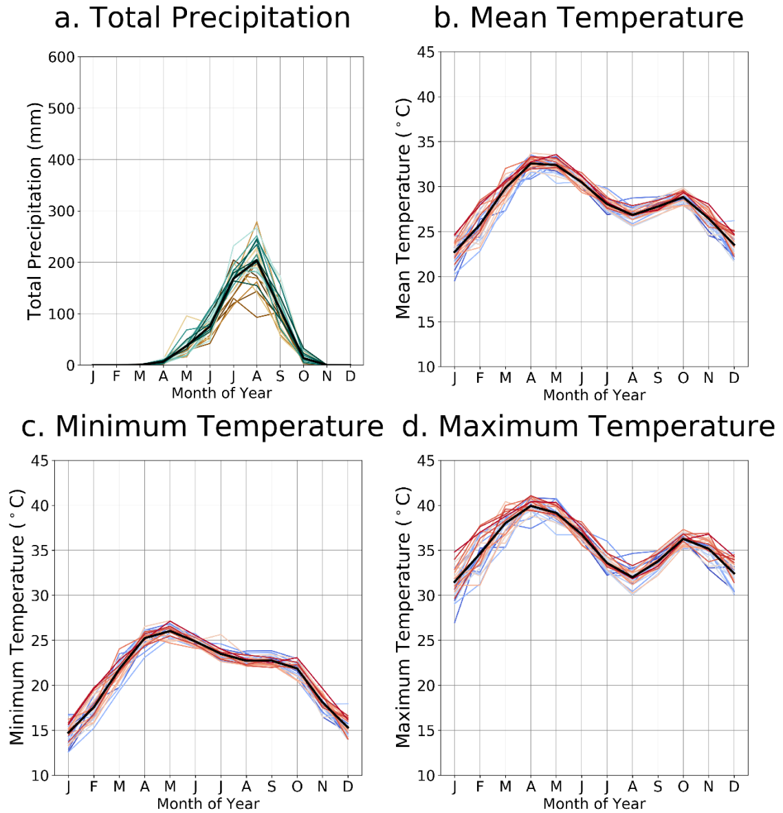
Figure B3: Observations for Zone 2 of total monthly precipitation (a) and average daily mean (b), minimum (c) and maximum (d) temperature over the baseline period (1981-2010). Precipitation data from CHIRPS (Climate Hazards group Infrared Precipitation with Stations) and temperature data from WFDEI-CRU (WATCH Forcing Data methodology applied to ERA-Interim data). Each line is one individual year. Colours show the ordering of years from brown to blue (total precipitation) and blue to red (mean temperature) – this highlights the presence, or lack of, a trend over the baseline period. The bold black line indicates the average of the 30-year period.
