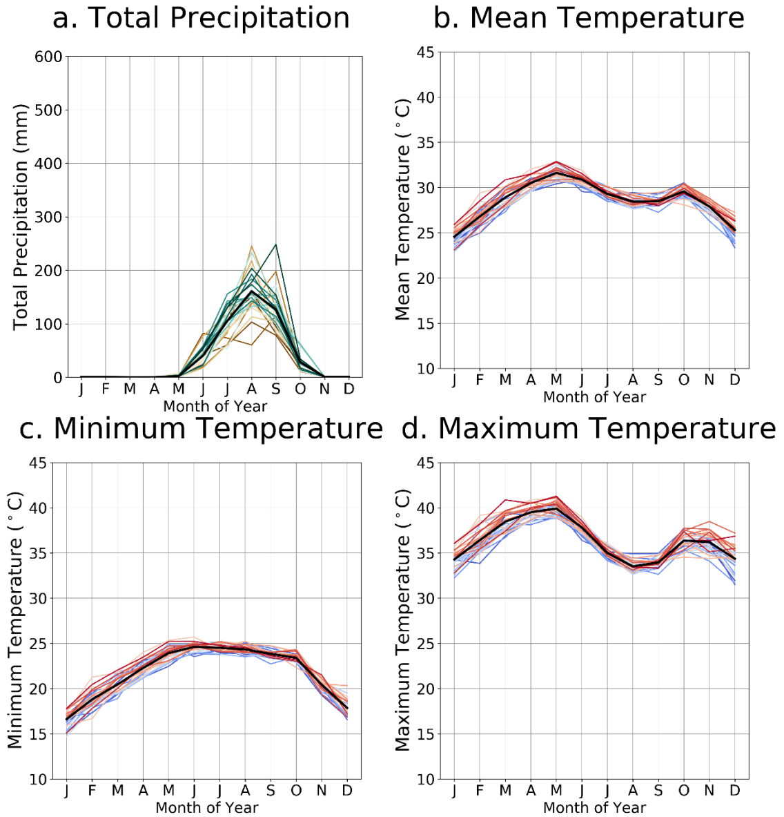
Figure B1: Observations for Zone 1 of total monthly precipitation (a) and average daily mean (b), minimum (c) and maximum (d) temperature over the baseline period (1981-2010). Precipitation data from CHIRPS (Climate Hazards group Infrared Precipitation with Stations) and temperature data from WFDEI-CRU (WATCH Forcing Data methodology applied to ERA-Interim data). Each line is one individual year. Colours show the ordering of years from brown to blue (total precipitation) and blue to red (mean temperature) – this highlights the presence, or lack of, a trend over the baseline period. The bold black line indicates the average of the 30-year period.
