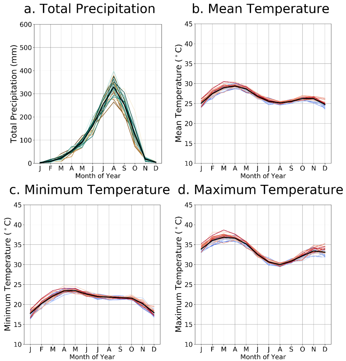
Figure B5: Observations for Zone 3 of total monthly precipitation (a) and average daily mean (b), minimum (c) and maximum (d) temperature over the baseline period (1981-2010). Precipitation data from CHIRPS (Climate Hazards group Infrared Precipitation with Stations) and temperature data from WFDEI-CRU (WATCH Forcing Data methodology applied to ERA-Interim data). Each line is one individual year. Colours show the ordering of years from brown to blue (total precipitation) and blue to red (mean temperature) – this highlights the presence, or lack of, a trend over the baseline period. The bold black line indicates the average of the 30-year period.
