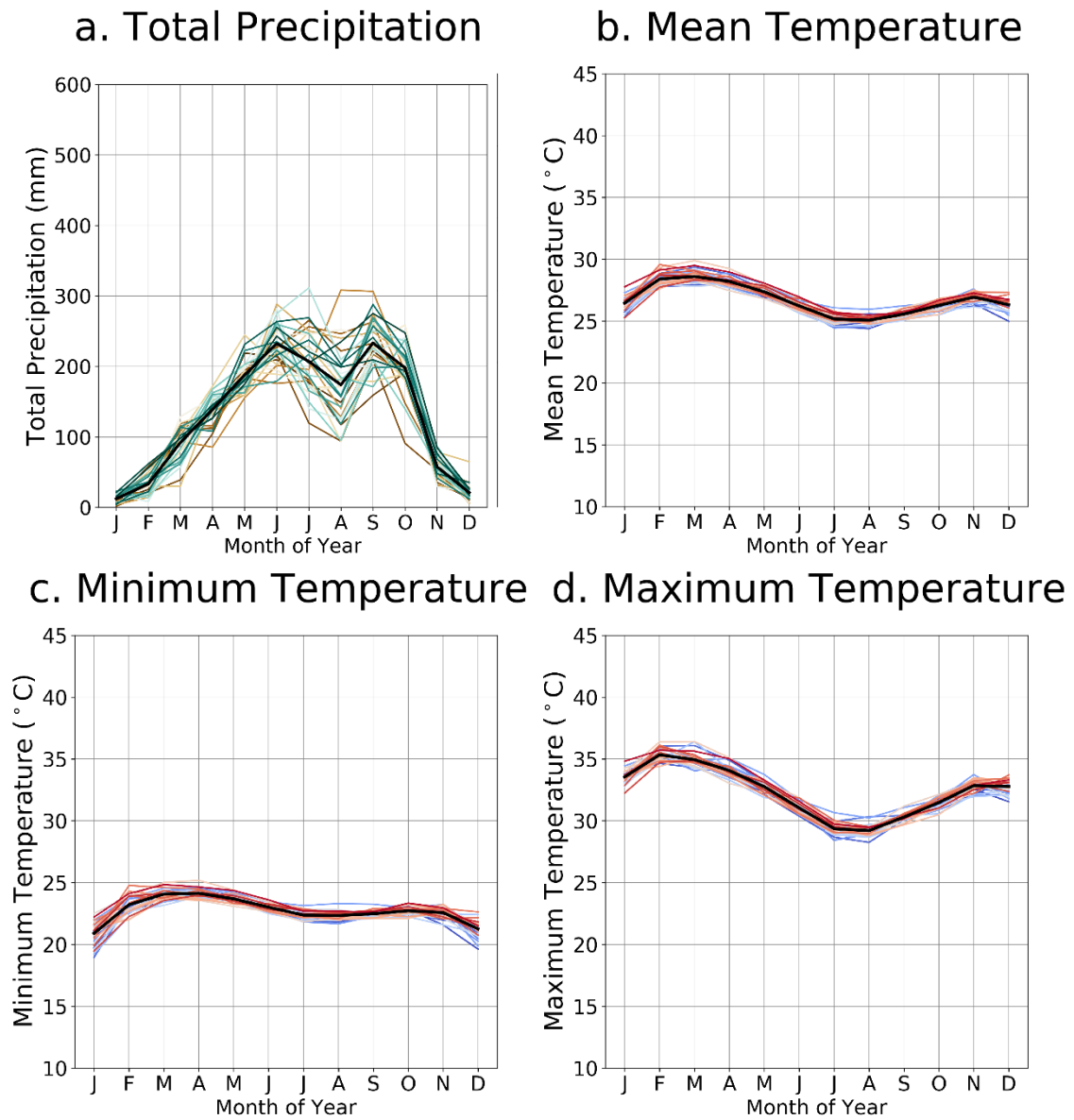
Figure B11: Observations for Zone 6 of total monthly precipitation (a) and average daily mean (b), minimum (c) and maximum (d) temperature over the baseline period (1981-2010). Precipitation data from CHIRPS (Climate Hazards group Infrared Precipitation with Stations) and temperature data from WFDEI-CRU (WATCH Forcing Data methodology applied to ERA-Interim data). Each line is one individual year. Colours show the ordering of years from brown to blue (total precipitation) and blue to red (mean temperature) – this highlights the presence, or lack of, a trend over the baseline period. The bold black line indicates the average of the 30-year period.
