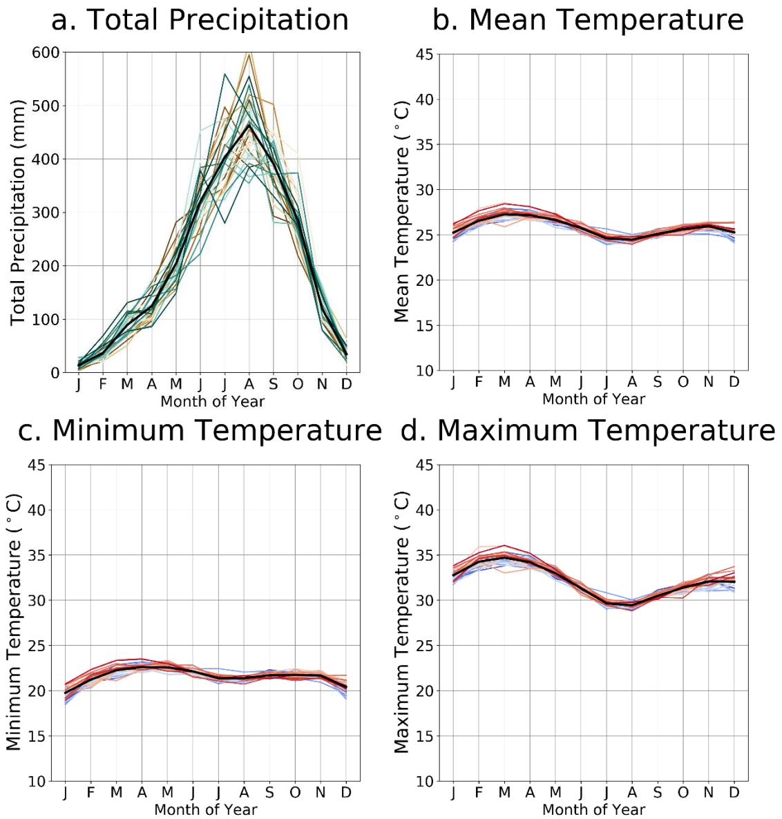
Figure B9: Observations for Zone 5 of total monthly precipitation (a) and average daily mean (b), minimum (c) and maximum (d) temperature over the baseline period (1981-2010). Precipitation data from CHIRPS (Climate Hazards group Infrared Precipitation with Stations) and temperature data from WFDEI-CRU (WATCH Forcing Data methodology applied to ERA-Interim data). Each line is one individual year. Colours show the ordering of years from brown to blue (total precipitation) and blue to red (mean temperature) – this highlights the presence, or lack of, a trend over the baseline period. The bold black line indicates the average of the 30-year period.
