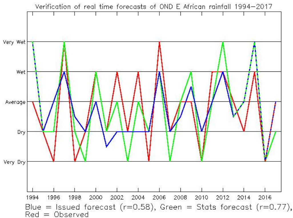
Figure 2.3: Verification of real time “best estimate” forecasts of October-December East African rainfall 1994-2017
