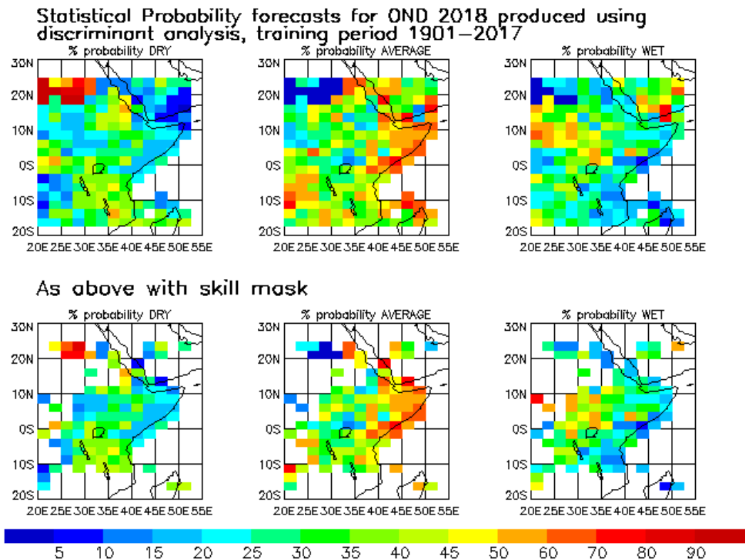
Figure 1.2a: Probability forecasts for the tercile categories obtained using the statistical method. The legend shows % probability, baseline for terciles is 1961-1990.
