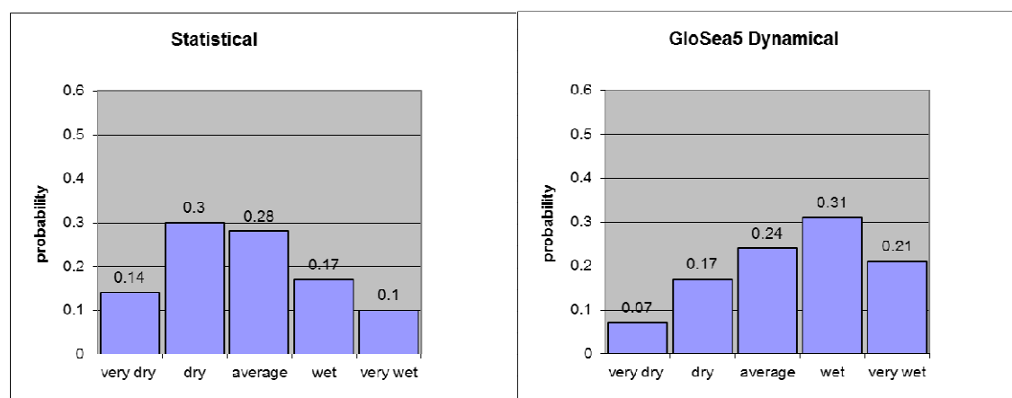
Figure 1.1: Predicted probabilities for October-November-December 2018 rainfall from the statistical and dynamical forecasts. Probabilities are for 5 quintile categories referred to as: very dry, dry, average, wet and very wet. The baseline (1961-1990) climatological probability for each category is by definition 0.2 (20%).
