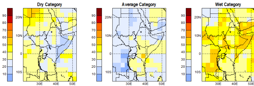
Figure 1.3: Probability forecasts for tercile categories obtained using the CCA-calibrated GloSea5. Baseline is 1981-2010
