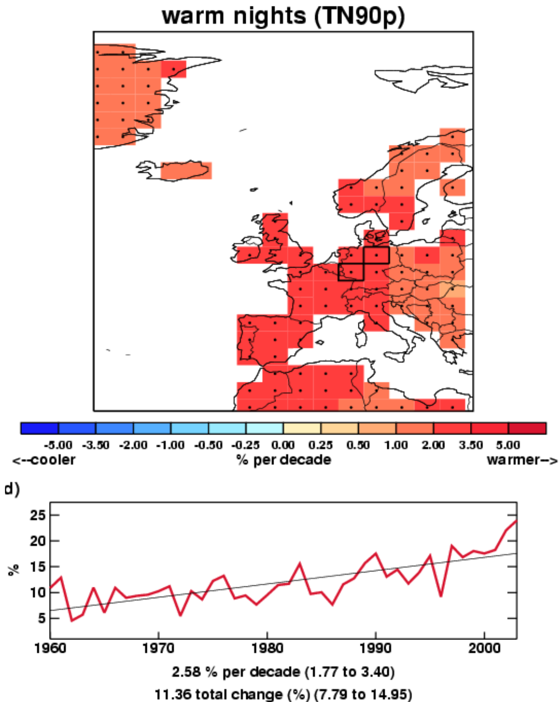
Figure 9. Examples of the plots shown in the data section. Left: From ECA&D data between 1960-2010 for the number of warm nights, and Right: from HadEX data (1960-2003) for the total precipitation. A full explanation of the plots is given in the text below.
