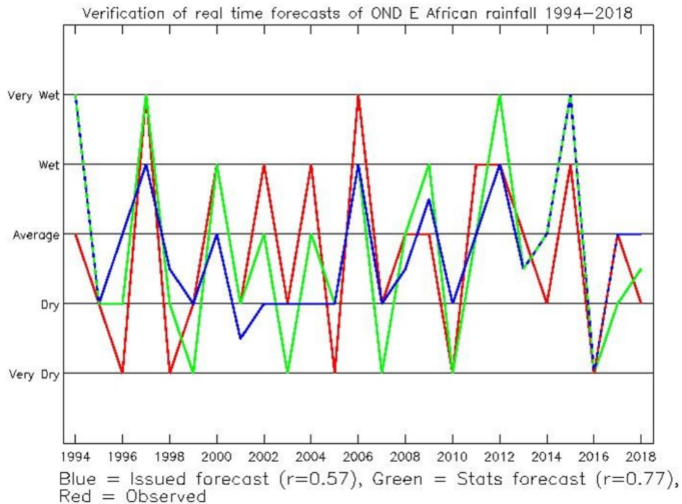
Figure 2.3: Verification of real time “best estimate” forecasts of October-December East African rainfall 1994-2018
