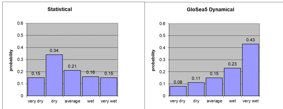
Figure 1.1: Predicted probabilities for October-November-December 2019 rainfall from the statistical and dynamical forecasts. Probabilities are for 5 quintile categories referred to as: very dry, dry, average, wet and very wet. The baseline (1961-1990) climatological probability for each category is by definition 0.2 (20%).
