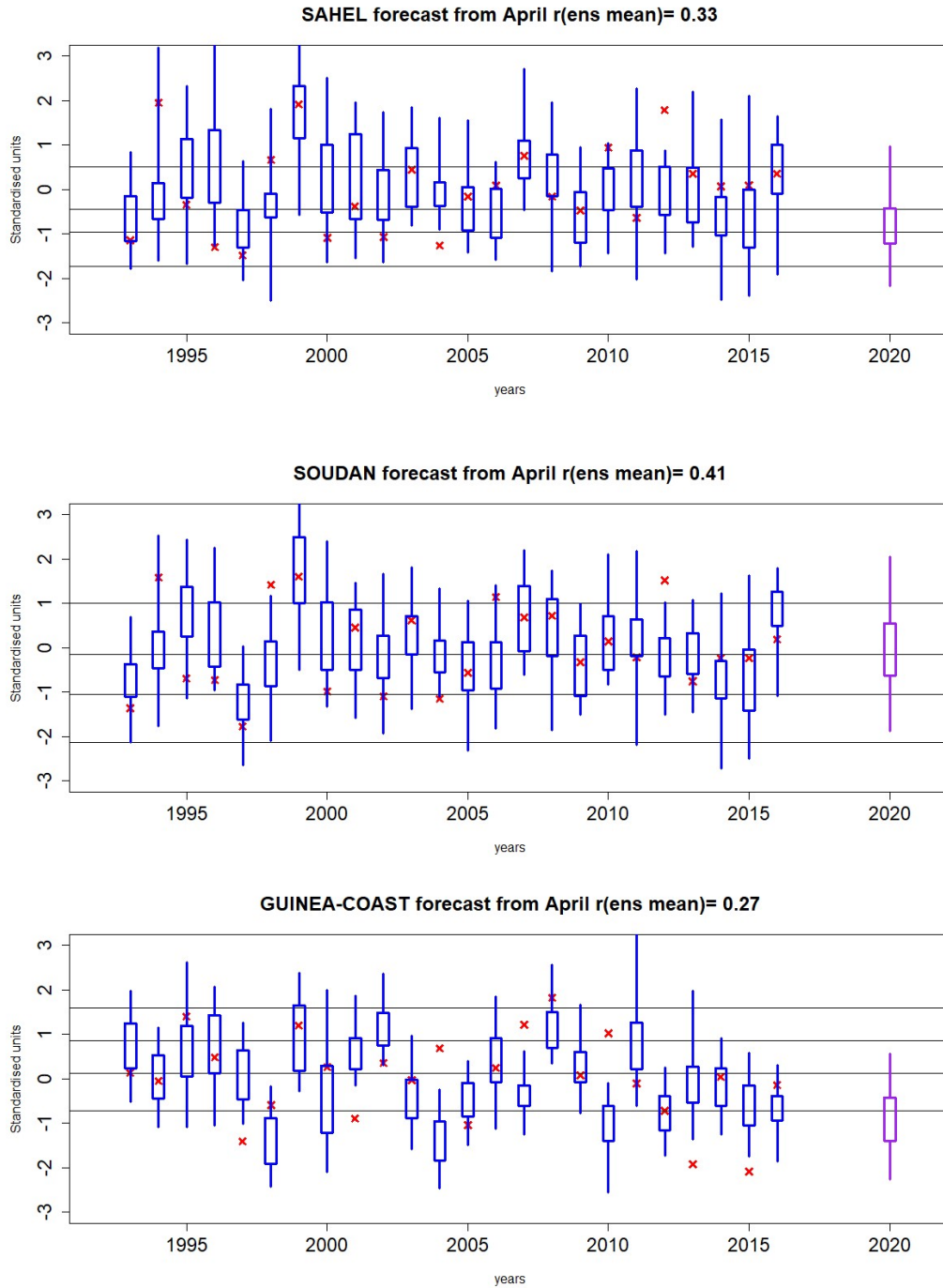
Figure 1.2: GloSea5 ensemble predictions for July-August-September 2020 (purple box-and-whisker far right) and corresponding retrospective forecasts (blue box-and-whisker) and observed rainfall (red crosses) for each year 1993-2016 and for the 3 North African regions. Solid horizontal lines are the quintile boundaries scaled as in Part 2.
