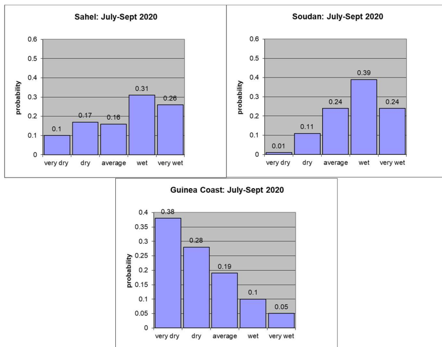
Figure 1.1: Predicted probabilities for July-August-September 2020 rainfall for the Sahel (15°W to 37.5°E, 12.5°N to 17.5°N); Soudan (7.5°W to 33.75°E, 10°N to 12.5°N) and Guinea Coast (7.5°W to 7.5°E, 5°N to 10°N) regions. Probabilities are for 5 categories referred to as: very dry, dry, average, wet and very wet. The category boundaries are defined from 1961-1990 observations, such that the climatological probability for each category in that period is by definition 0.2 (20%).
