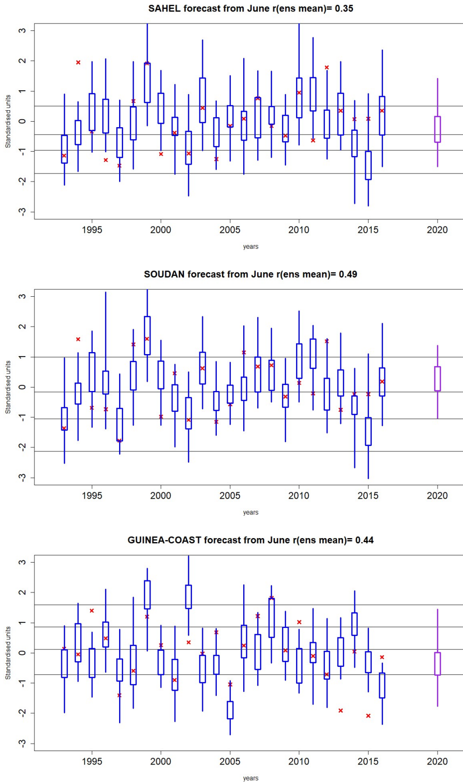
Figure 1.2: GloSea5 ensemble predictions for July-August-September 2020 (purple box-and-whisker far right) and corresponding retrospective forecasts (blue box-and-whisker) and observed rainfall (red crosses) for each year 1993-2016 and for the 3 North African regions. Solid horizontal lines are the quintile boundaries scaled as in Part 2.
