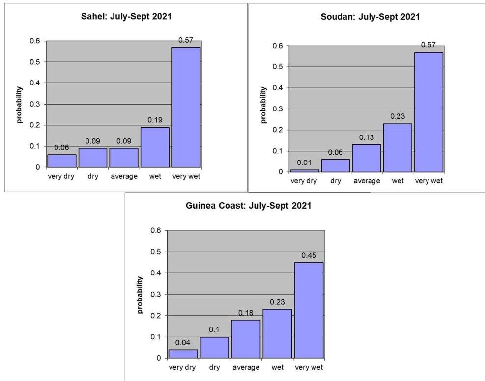
Figure 1.1: Predicted probabilities for July-August-September 2021 rainfall for the Sahel (15°W to 37.5°E, 12.5°N to 17.5°N); Soudan (7.5°W to 33.75°E, 10°N to 12.5°N) and Guinea Coast (7.5°W to 7.5°E, 5°N to 10°N) regions. Probabilities are for 5 categories referred to as: very dry, dry, average, wet and very wet. The category boundaries are defined from 1961-1990 observations, such that the climatological probability for each category in that period is by definition 0.2 (20%).
