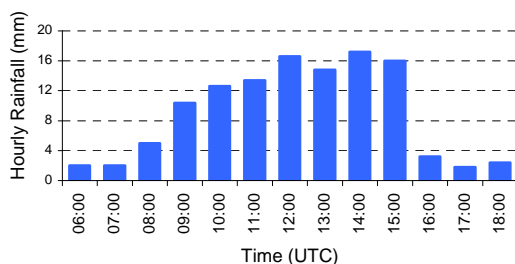
Hourly rainfall totals for Brize Norton
