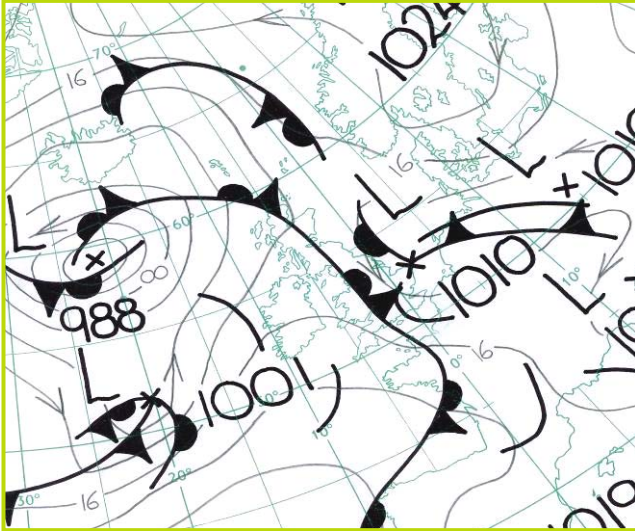
Weather chart for 1200 UTC on 3 June 2008
