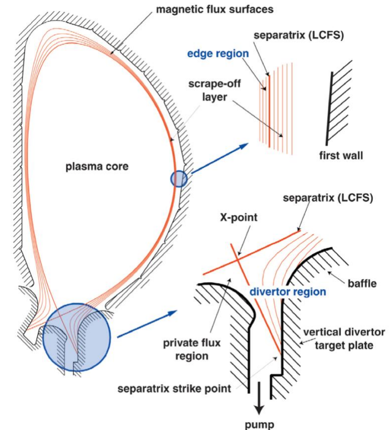
Figure 1: Schematic diagram of a generic tokamak “poloidal cross section” showing the areas of plasma and first wall that will be targeted by project NEPTUNE (shaded circles). Attribution: G. Federici et al. [CC BY 3.0 ( https://creativecommons.org/licenses/by/3.0/ )]†.
