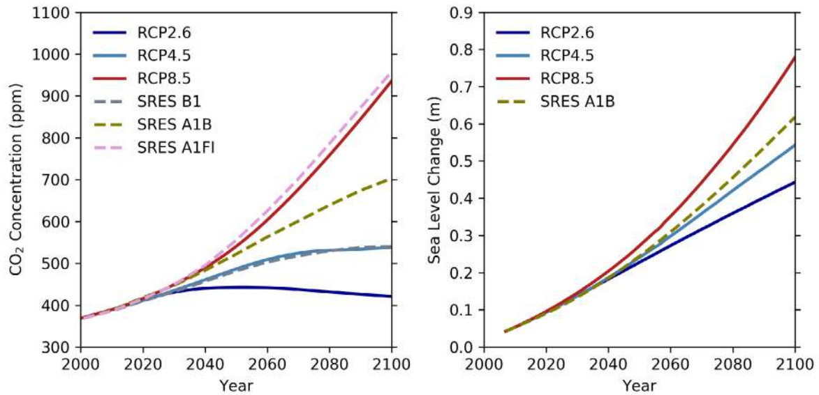
Figure 5.1.1. (left) Time series of CO 2 concentrations over the 21 st century for the RCP scenarios (Meinshausen et al, 2011) and SRES scenarios ( https://www.ipcc.ch/reports/ ) based on the Bern-CC Model. (right) The corresponding central estimates of time-mean sea level rise over the 21 st century using UKCP18 methods for all available scenarios. The SRES A1B projection makes uses the projections of Antarctic ice dynamics from RCP4.5, but the results are not sensitive to the choice of scenario.
