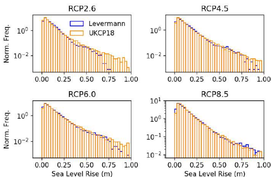
Figure A1.1.1. Comparison of the normalised frequency distribution of sea level rise from Antarctic ice dynamics at 2100, from: Levermann et al, (2014; blue); UKCP18 log-normal fit (orange). Note the log-scale on the Y-axis.
