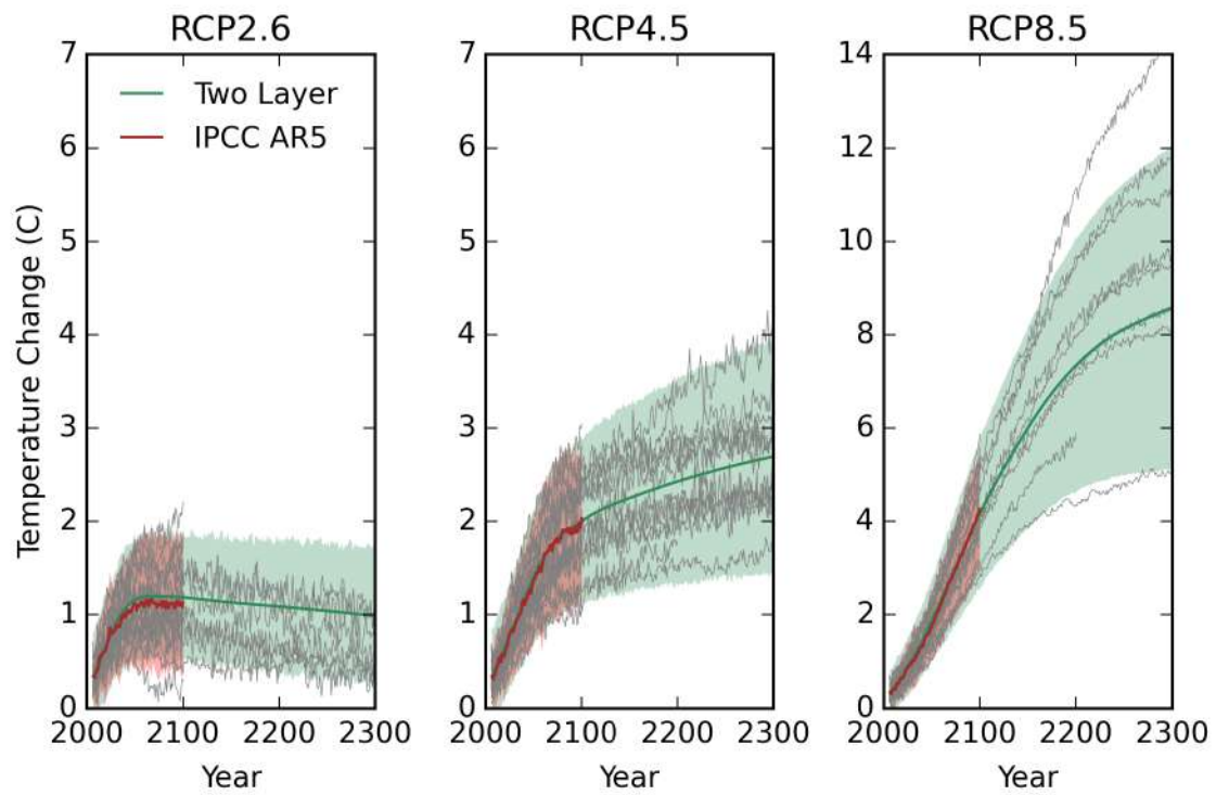
Figure A1.2.2. Ensemble projections of global surface temperature change (C) relative to a baseline period of 1986–2005. Time series include: (i) the 21-member CMIP5 ensemble used for sea level projections in IPCC AR5 (red, shaded regions indicate 5 th to 95 th percentile range); (ii) the 14 member two-layer model ensemble (green, shaded regions indicate 5 th to 95 th percentile range); (iii) individual CMIP5 model projections (grey lines). Figure reproduced from Palmer et al, (2018).
