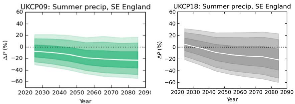
Figure 2: Probabilistic projections of summer average precipitation (%), \Delta P , from UKCP09 (left) and UKCP18 (right), for the SRES A1B emissions scenario for the South East England administrative region. The white line shows the median (50 th percentile) of the probability distribution and shading shows the 5 th , 10 th , 25 th , 75 th , 90 th and 95 th percentiles. Changes in 30-year averages are shown relative to the UKCP09 baseline of 1961-1990, for the seven overlapping future periods provided in UKCP09: 2011-2040, 2021-2050, 2071-2100 (based on Figure 2.6 of Murphy et al, 2018).
