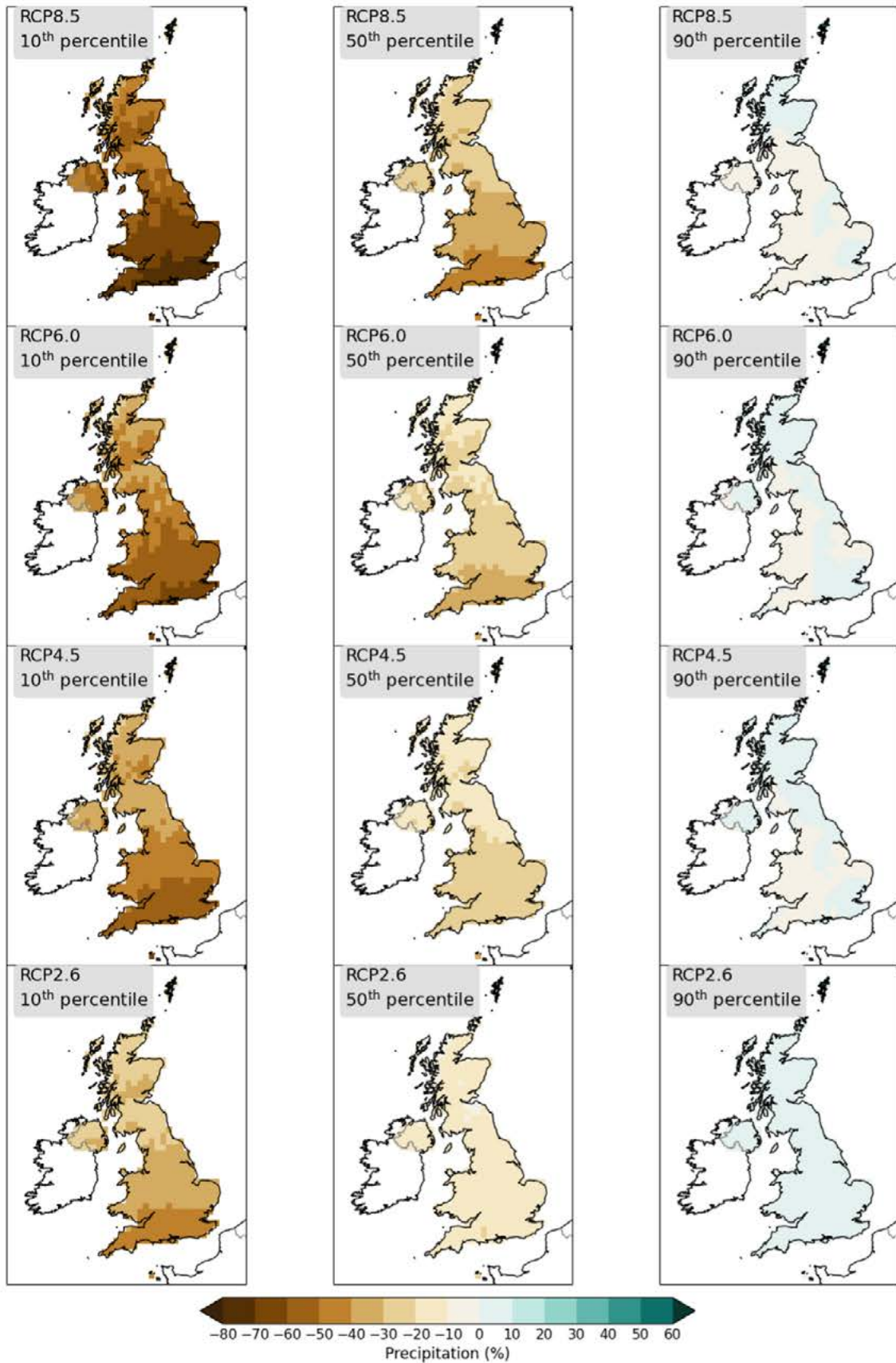
Figure 1. Projected changes in summer mean precipitation for the UK for 2080-2099 compared to 1981-2000 using the probabilistic projections. RCP2.6 is the lowest emissions scenario and RCP8.5 is the highest emissions scenario.
