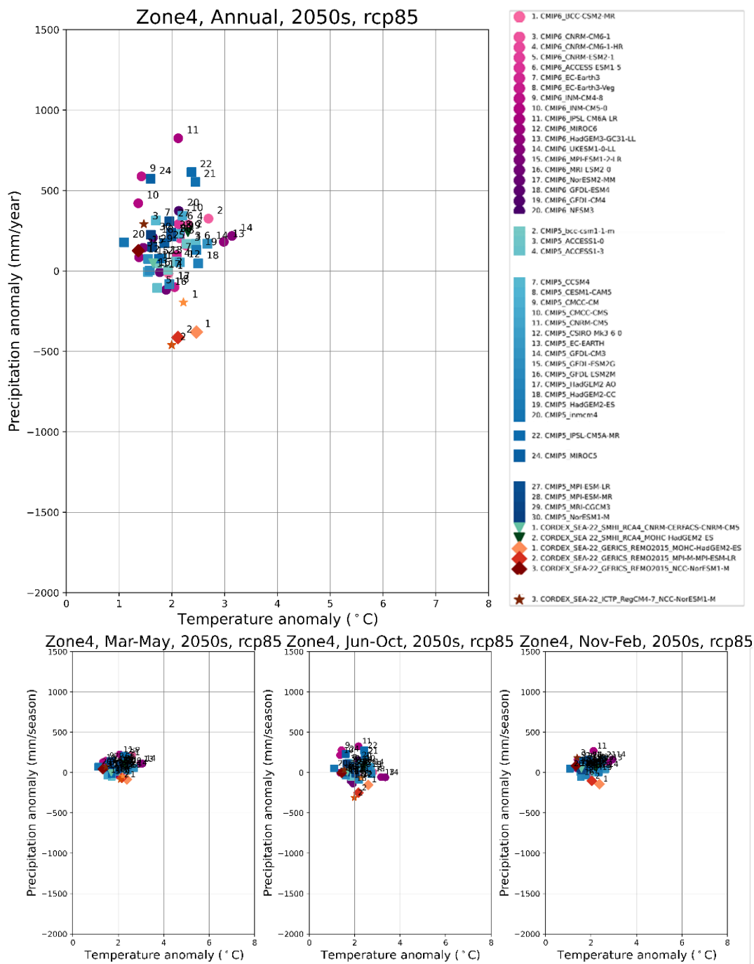
Figure E16: Projected change in average annual (top panel) and seasonal (bottom panels) precipitation and temperature in Zone 4. Each dot shows the difference between the average projected values in the 2050s and the average values in the current climate, for each climate model. Individual models are identified by the icon and number in the legend.
