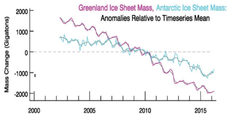
Fig 1 - Changes in the mass of the Greenland and Antarctic ice sheets from the satellite gravity mission GRACE. Source: NASA GRACE, David Wiese, JPL
