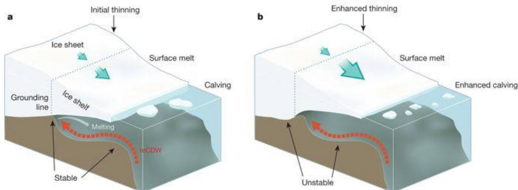
Fig 2 - Marine ice sheet instability occurs when the edge of the ice sheet rests on bedrock that deepens inland, as shown in panel b). A warming ocean melts the ice, causing the ice sheet edge to retreat. This exposes a greater depth of ice to loss into the ocean, driving further retreat (11)
