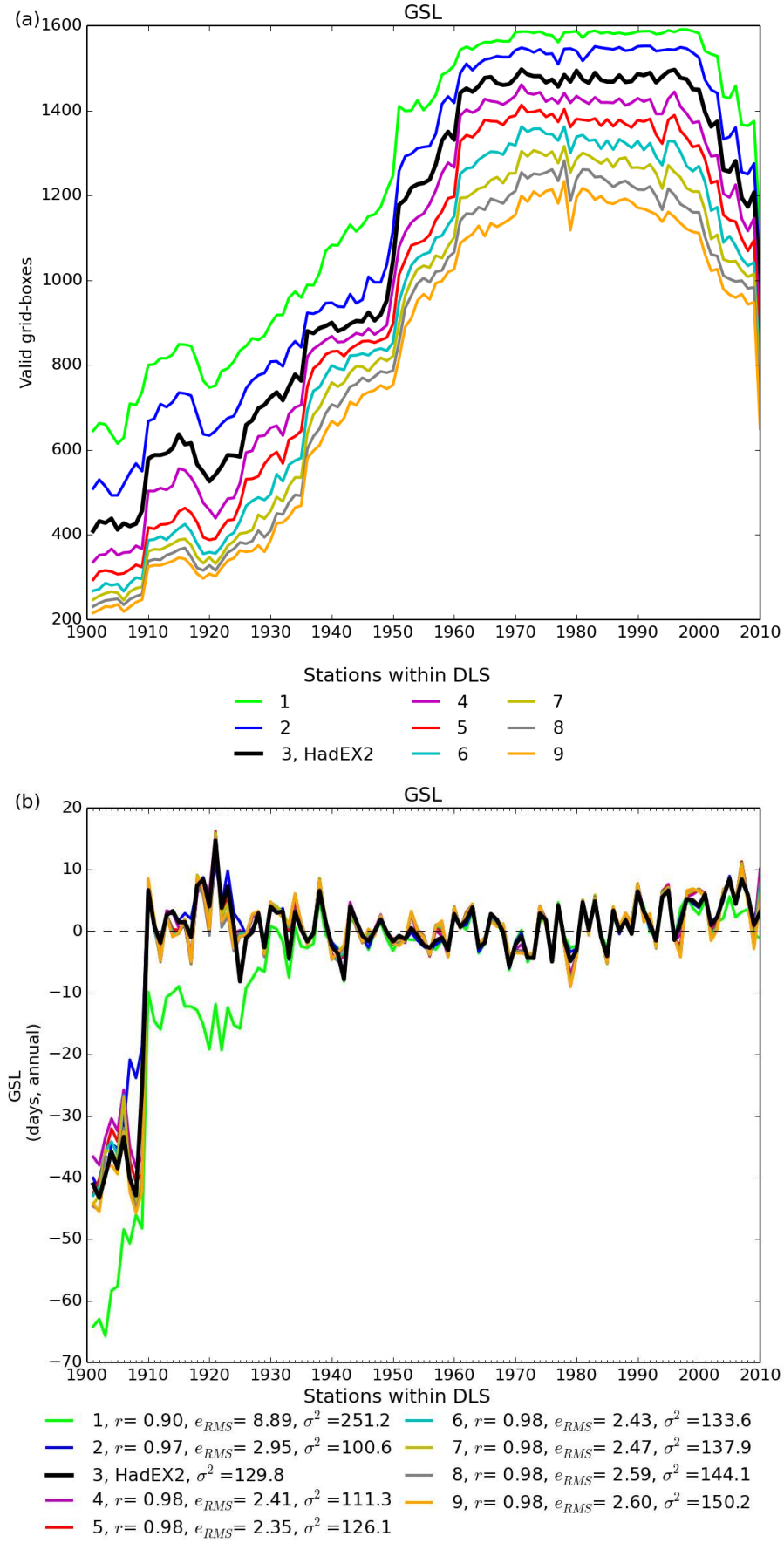
Figure 3: (a) : The number of non-missing grid boxes for GSL showing the different curves for left numbers of stations within a DLS of the grid box centre. Note that the global average only takes grid boxes which have 90 per cent completeness or more, whereas all grid boxes are shown in the coverage series. (b) : The time series for global average GSL.
