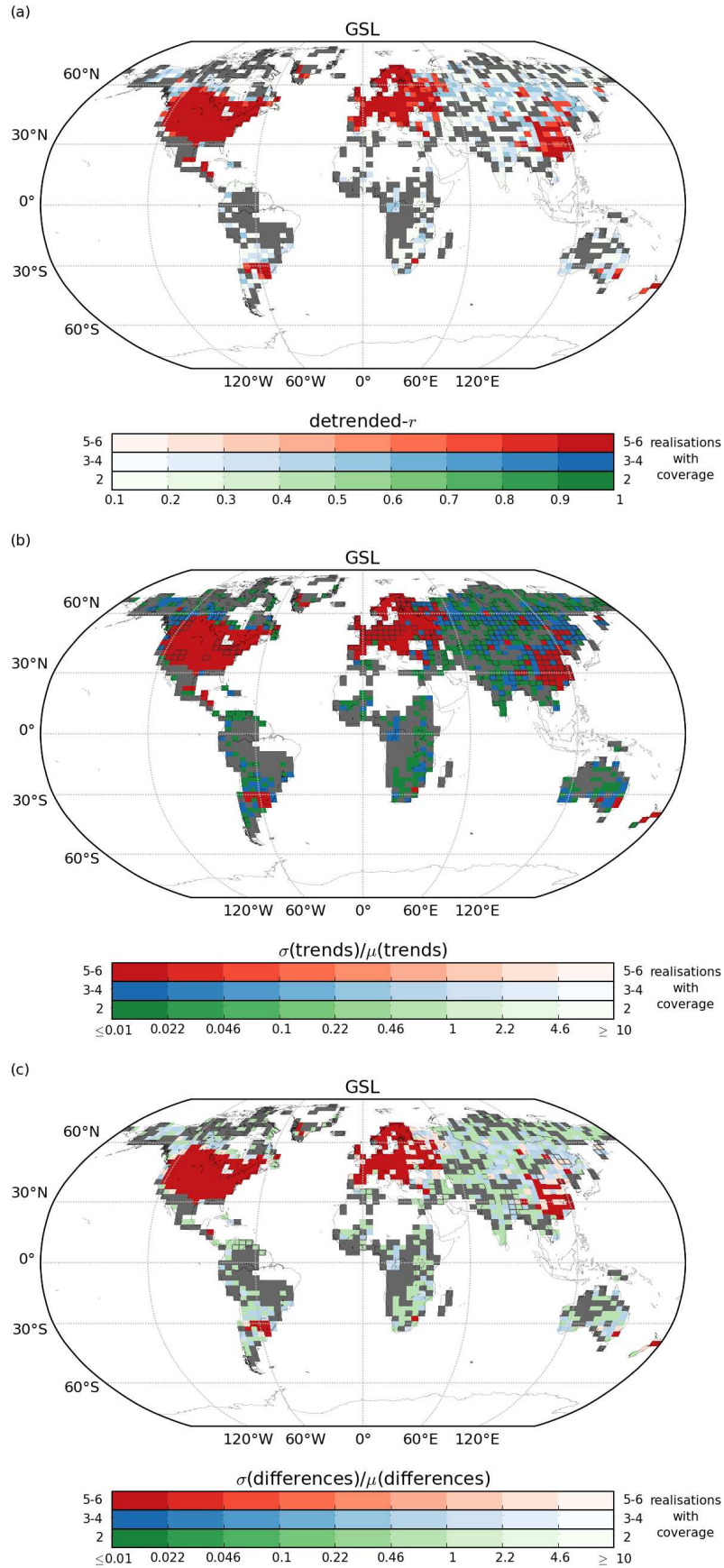
Figure 6: As for Fig. 4 but for GSL restricted by the number of stations within a grid box. Grey grid boxes are those where only one of the 6 possible stations per grid box choices results in a value, green when 2, blue when 3-4 and red when 5-6 of the possible choices result in a value. Note that the HadEX2 method does not require any stations to be present within a grid box for a value to be calculated. In (b) and (c), boxes which have been outlined are ones where the trend was significant in the HadEX2 version. For details on the calculation method, see text.
