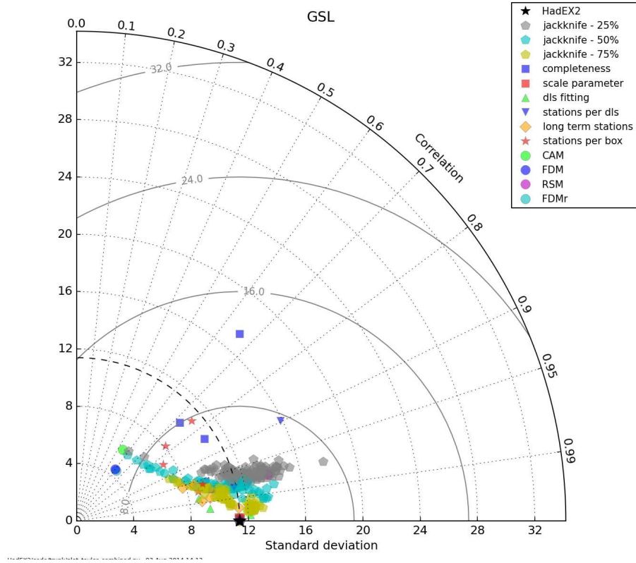
Figure 19: The Taylor Diagram for GSL calculated using the global average timeseries for each choice. Each of the different methodological choices are shown using a different symbol and colour as indicated in the legend.
