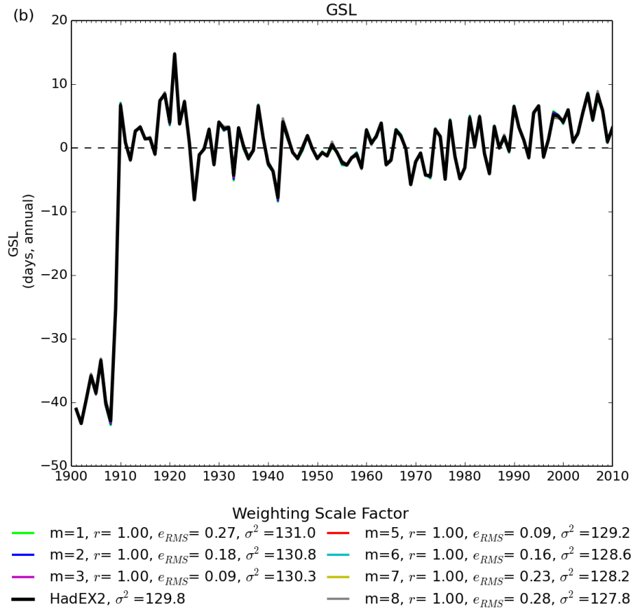
Figure 2: The time series for global average GSL showing the different curves for the different weighting values (colours are indicated below the plot). The figure also shows the correlation coefficient ( r ), variance ( \sigma^2 ) and root-mean-square error ( e_{RMS} ) between each series and HadEX2. All choices have been normalised over the 1961-1990 period.
