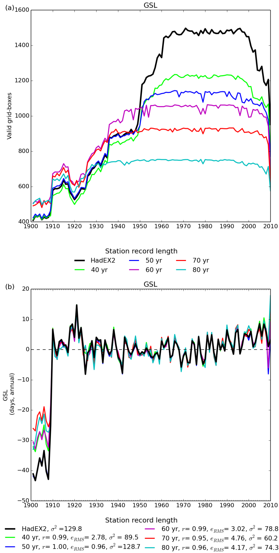
10 Figure 9: As for Fig. 3 but for long-term stations.
