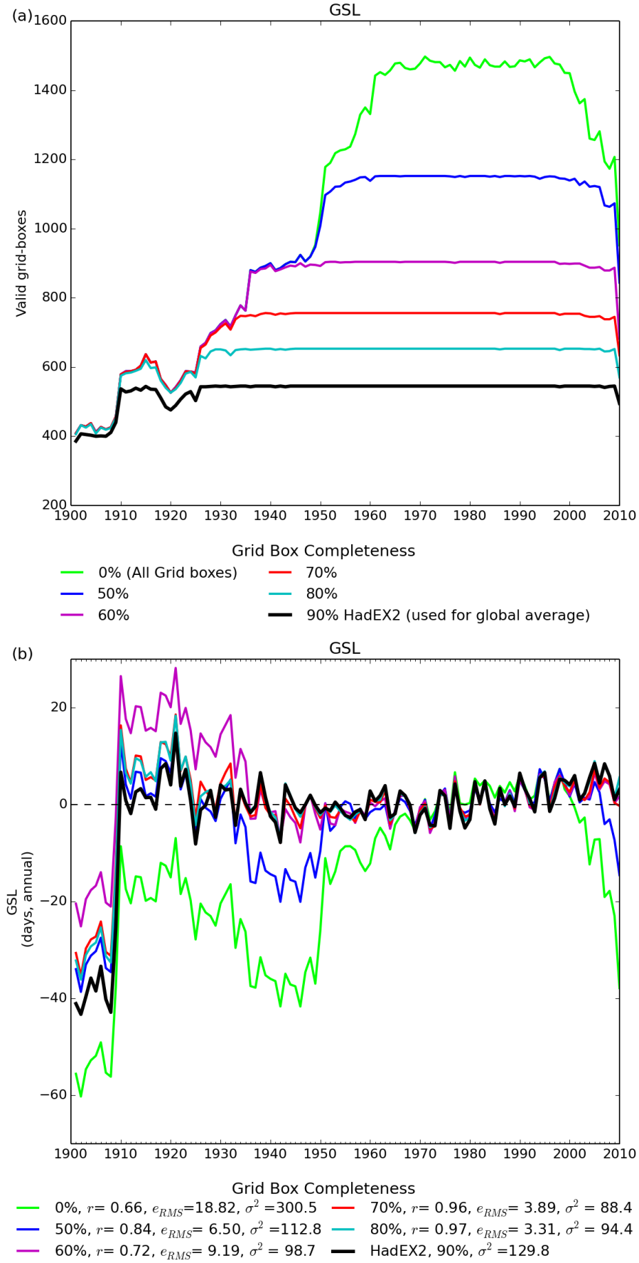
Figure 1: (a) The coverage, showing the different curves for different completeness requirements, for GSL. The total coverage is shown the curve in light green, whereas the coverage used when calculating global averages is in black, with a range of other completeness percentages shown in between. (b) : The time series for global average of GSL. Also shown are the comparison of other completenesses to that used in HadEX2 (90 %) using the correlation coefficient, r , the root mean square error e_{rms} and the variance, \sigma^2 .
