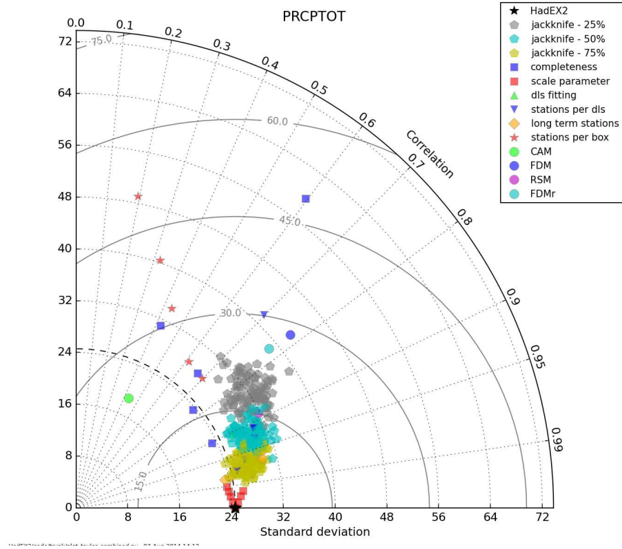
Figure 19: The Taylor Diagram for PRCPTOT calculated using the global average timeseries for each choice. Each of the different methodological choices are shown using a different symbol and colour as indicated in the legend.
