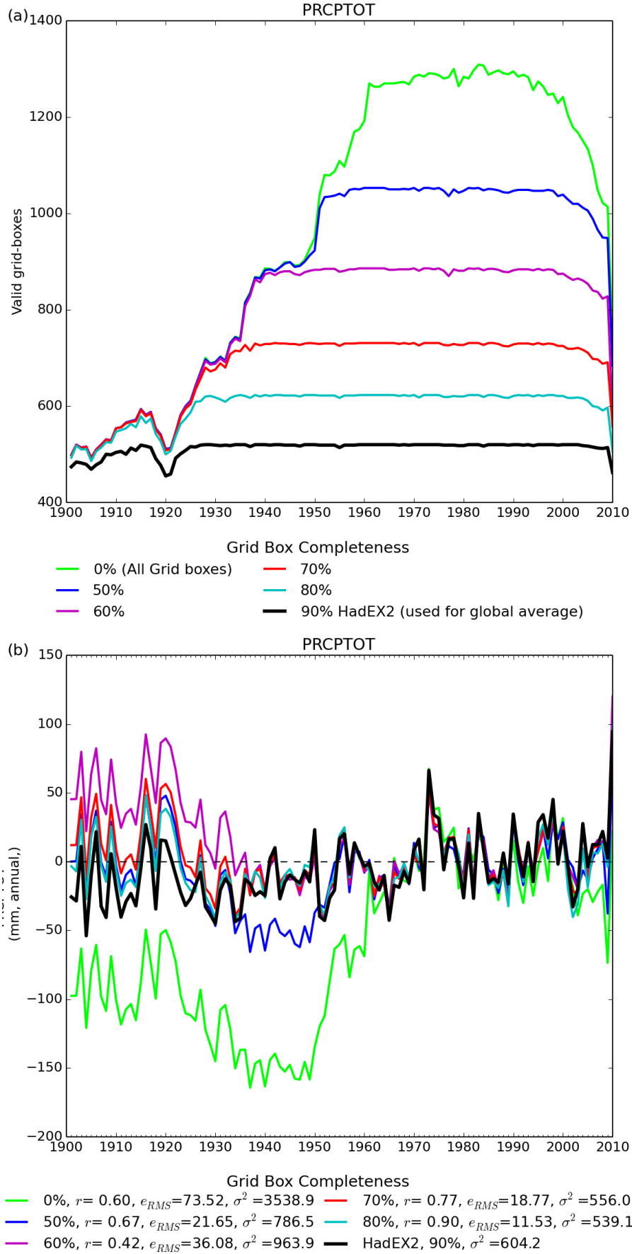
Figure 1: (a) The coverage, showing the different curves for different completeness requirements, for PRCPTOT. The total coverage is shown the curve in light green, whereas the coverage used when calculating global averages is in black, with a range of other completeness percentages shown in between. (b): The time series for global average of PRCPTOT. Also shown are the comparison of other completenesses to that used in HadEX2 (90 %) using the correlation coefficient, r , the root mean square error e_{ems} and the variance, \sigma^2 .
