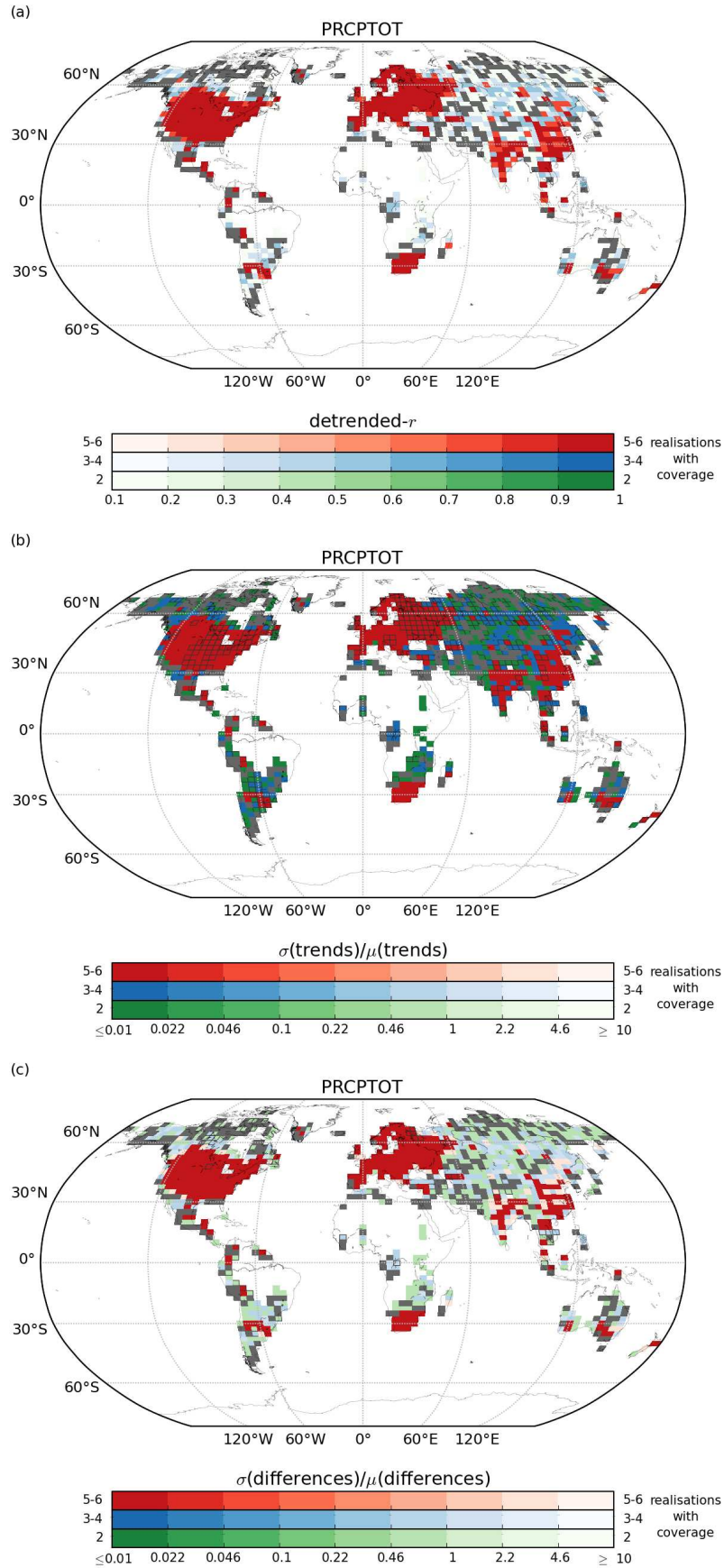
Figure 6: As for Fig. 4 but for PRCPTOT restricted by the number of stations within a grid box. Grey grid boxes are those where only one of the 6 possible stations per grid box choices results in a value, green when 2, blue when 3-4 and red when 5-6 of the possible choices result in a value. Note that the HadEX2 method does not require any stations to be present within a grid box for a value to be calculated. In (b) and (c), boxes which have been outlined are ones where the trend was significant in the HadEX2 version. For details on the calculation method, see text.
