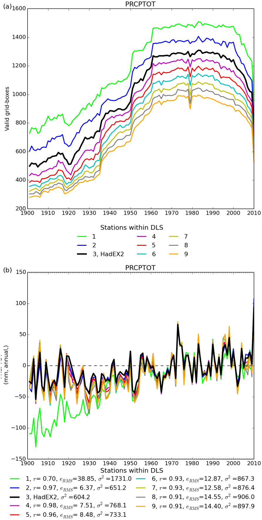
Figure 3: (a) : The number of non-missing grid boxes for PRCPTOT showing the different curves for left numbers of stations within a DLS of the grid box centre. Note that the global average only takes grid boxes which have 90 per cent completeness or more, whereas all grid boxes are shown in the coverage series. (b) : The time series for global average PRCPTOT.
