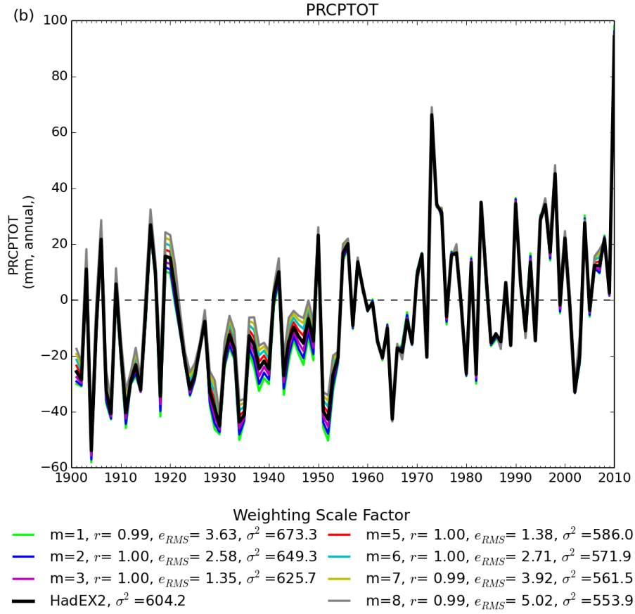
Figure 2: The time series for global average PRCPTOT showing the different curves for the different weighting values (colours are indicated below the plot). The figure also shows the correlation coefficient ( r ), variance ( \sigma^2 ) and root-mean-square error ( e_{RMS} ) between each series and HadEX2. All choices have been normalised over the 1961-1990 period.
