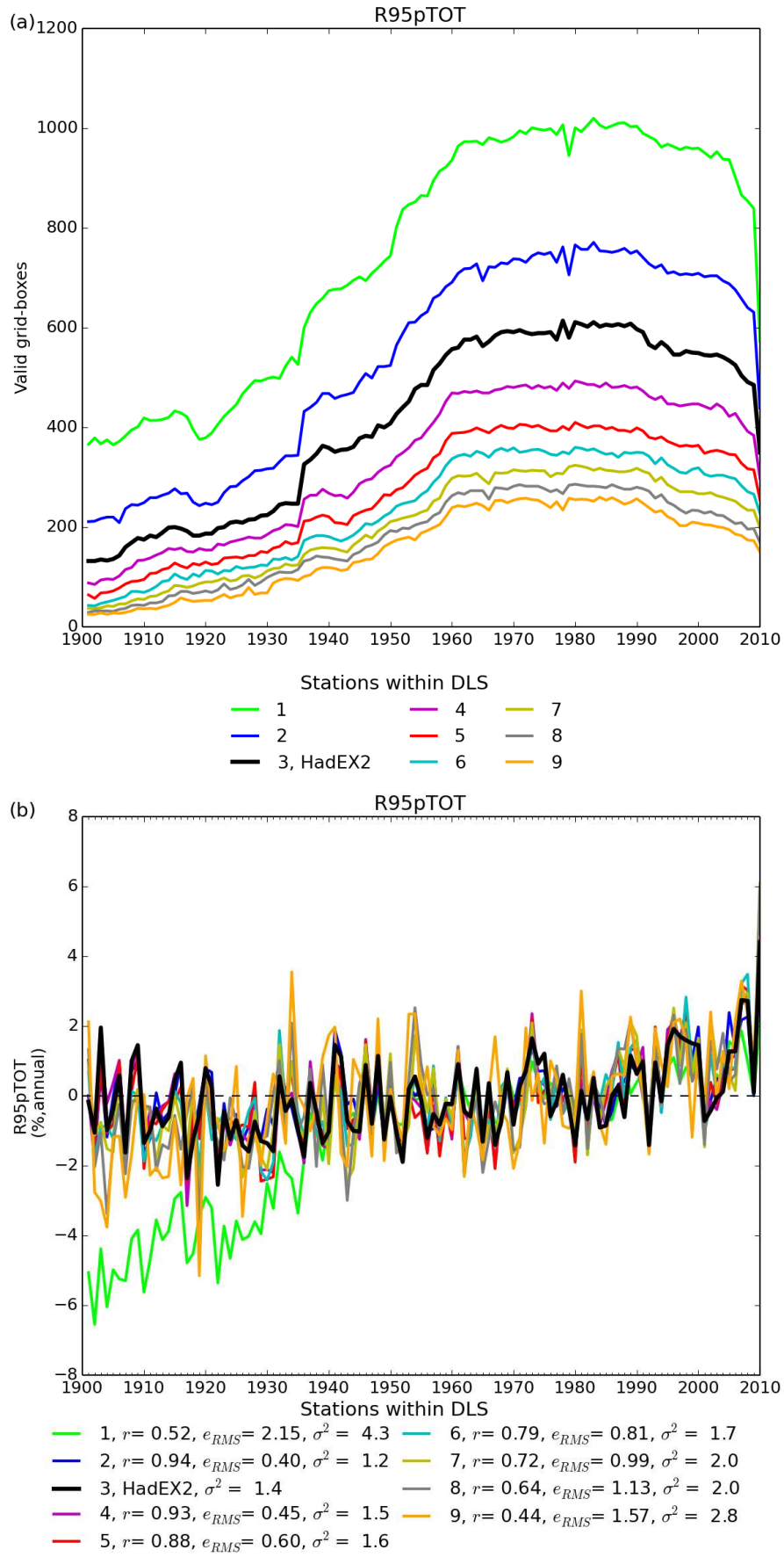
Figure 3: (a) : The number of non-missing grid boxes for R95pTOT showing the different curves for left numbers of stations within a DLS of the grid box centre. Note that the global average only takes grid boxes which have 90 per cent completeness or more, whereas all grid boxes are shown in the coverage series. (b) : The time series for global average R95pTOT.
