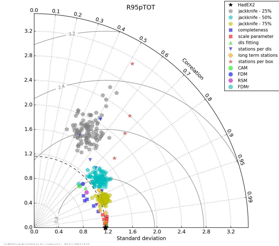
Figure 19: The Taylor Diagram for R95pTOT calculated using the global average timeseries for each choice. Each of the different methodological choices are shown using a different symbol and colour as indicated in the legend.
