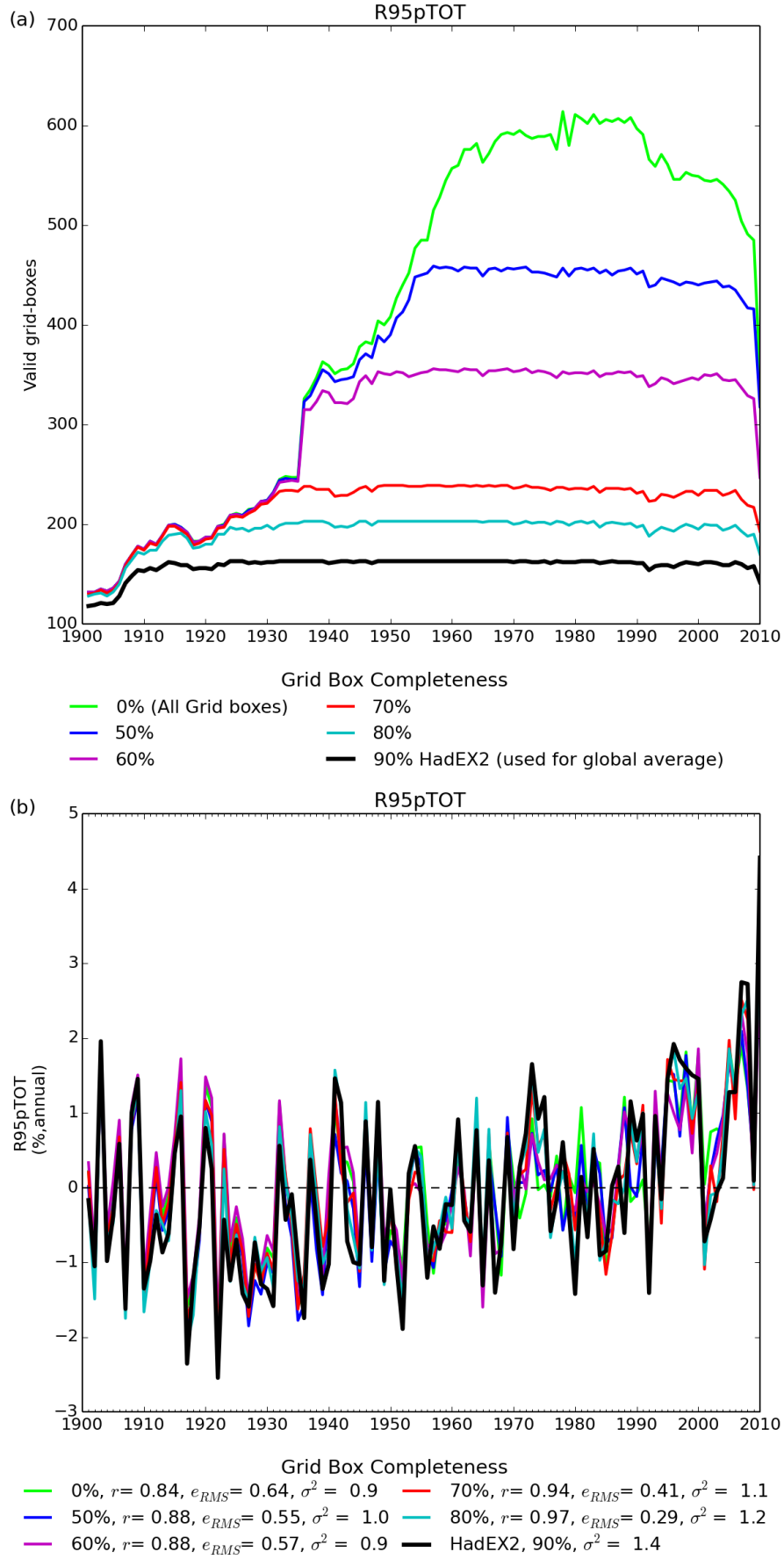
Figure 1: (a) The coverage, showing the different curves for different completeness requirements, for R95pTOT. The total coverage is shown the curve in light green, whereas the coverage used when calculating global averages is in black, with a range of other completeness percentages shown in between. (b): The time series for global average of R95pTOT. Also shown are the comparison of other completenesses to that used in HadEX2 (90 %) using the correlation coefficient, r , the root mean square error e_{ems} and the variance, \sigma^2 .
