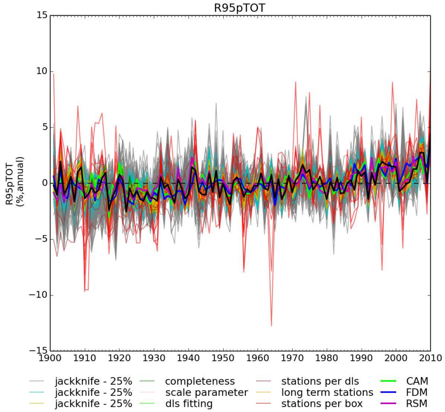
Figure 18: The timeseries curves for all of the different methodological choices assessed during this work, with HadEX2 shown by the thick black line.
