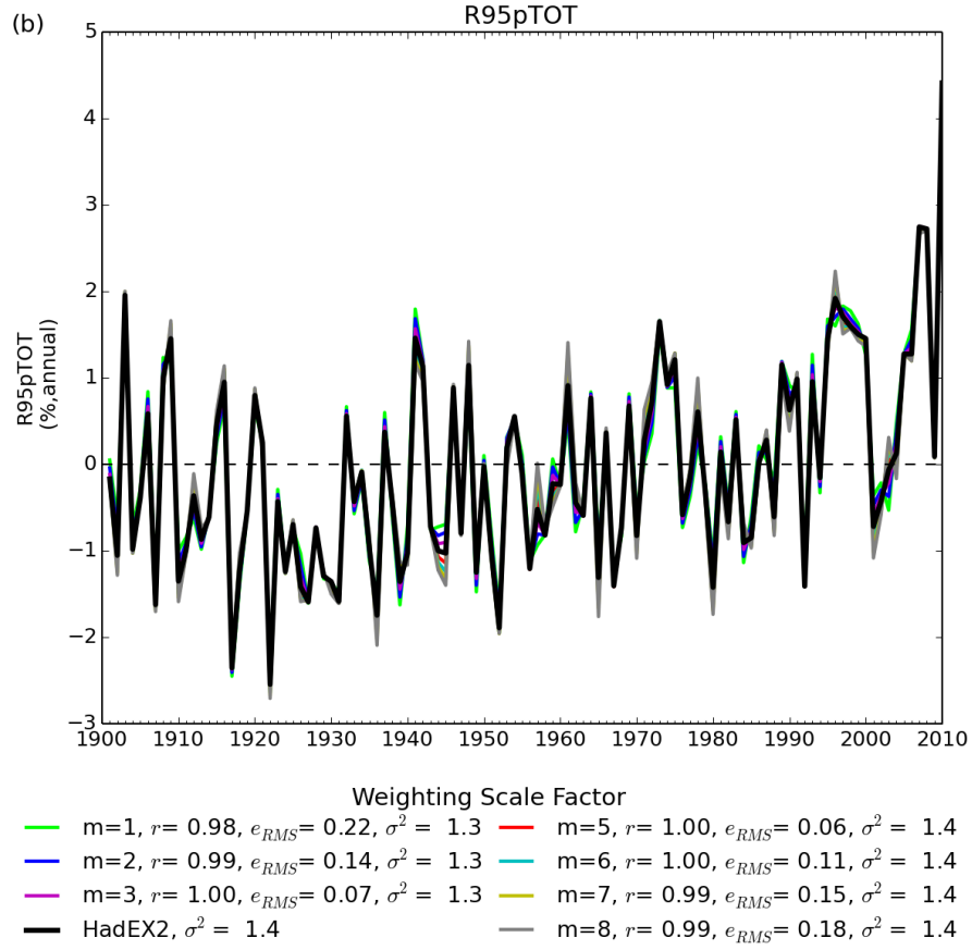
Figure 2: The time series for global average R95pTOT showing the different curves for the different weighting values (colours are indicated below the plot). The figure also shows the correlation coefficient ( r ), variance ( \sigma^2 ) and root-mean-square error ( e_{RMS} ) between each series and HadEX2. All choices have been normalised over the 1961-1990 period.
