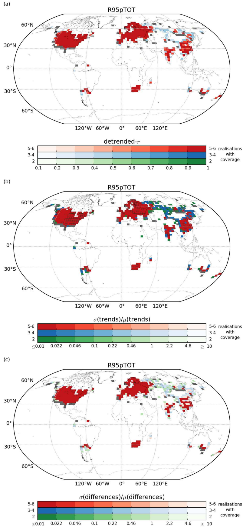
Figure 6: As for Fig. 4 but for R95pTOT restricted by the number of stations within a grid box. Grey grid boxes are those where only one of the 6 possible stations per grid box choices results in a value, green when 2, blue when 3-4 and red when 5-6 of the possible choices result in a value. Note that the HadEX2 method does not require any stations to be present within a grid box for a value to be calculated. In (b) and (c), boxes which have been outlined are ones where the trend was significant in the HadEX2 version. For details on the calculation method, see text.
