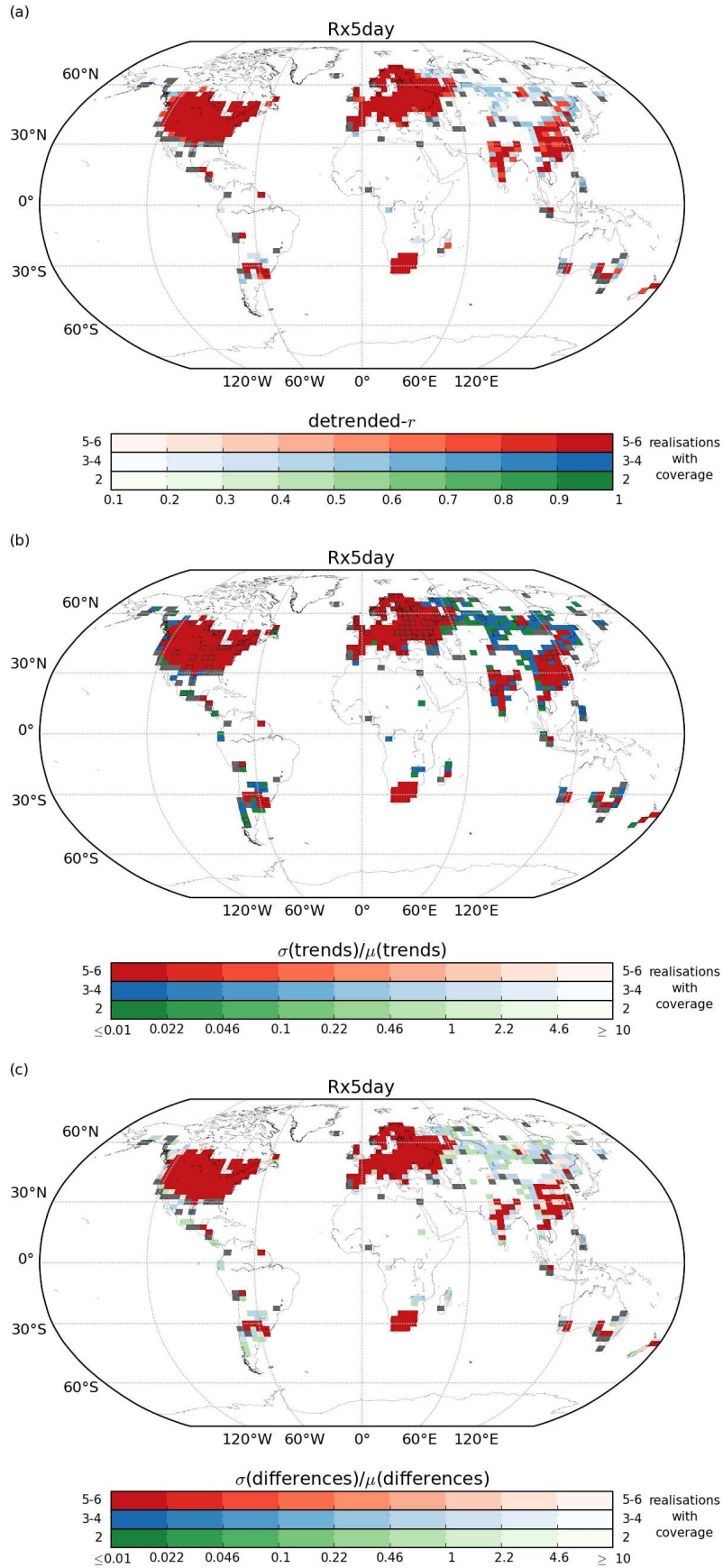
Figure 6: As for Fig. 4 but for Rx5day restricted by the number of stations within a grid box. Grey grid boxes are those where only one of the 6 possible stations per grid box choices results in a value, green when 2, blue when 3-4 and red when 5-6 of the possible choices result in a value. Note that the HadEX2 method does not require any stations to be present within a grid box for a value to be calculated. In (b) and (c), boxes which have been outlined are ones where the trend was significant in the HadEX2 version. For details on the calculation method, see text.
