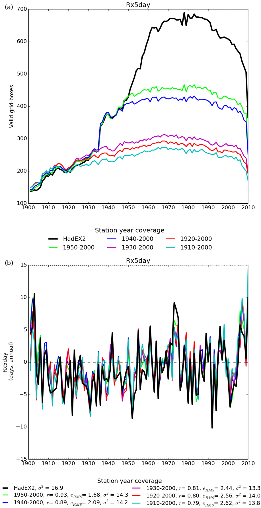
Figure 7: As for Fig. 3 but for long-term stations selected using five time periods as detailed in the legend
