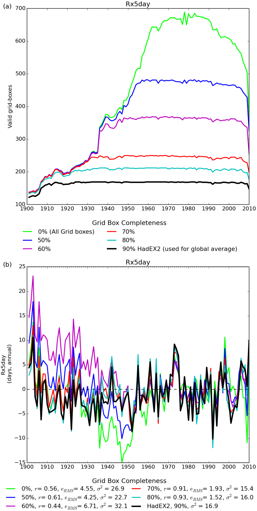
Figure 1: (a) The coverage, showing the different curves for different completeness requirements, for Rx5day. The total coverage is shown the curve in light green, whereas the coverage used when calculating global averages is in black, with a range of other completeness percentages shown in between. (b): The time series for global average of Rx5day. Also shown are the comparison of other completenesses to that used in HadEX2 (90 %) using the correlation coefficient, r , the root mean square error e_{ems} and the variance, \sigma^2 .
