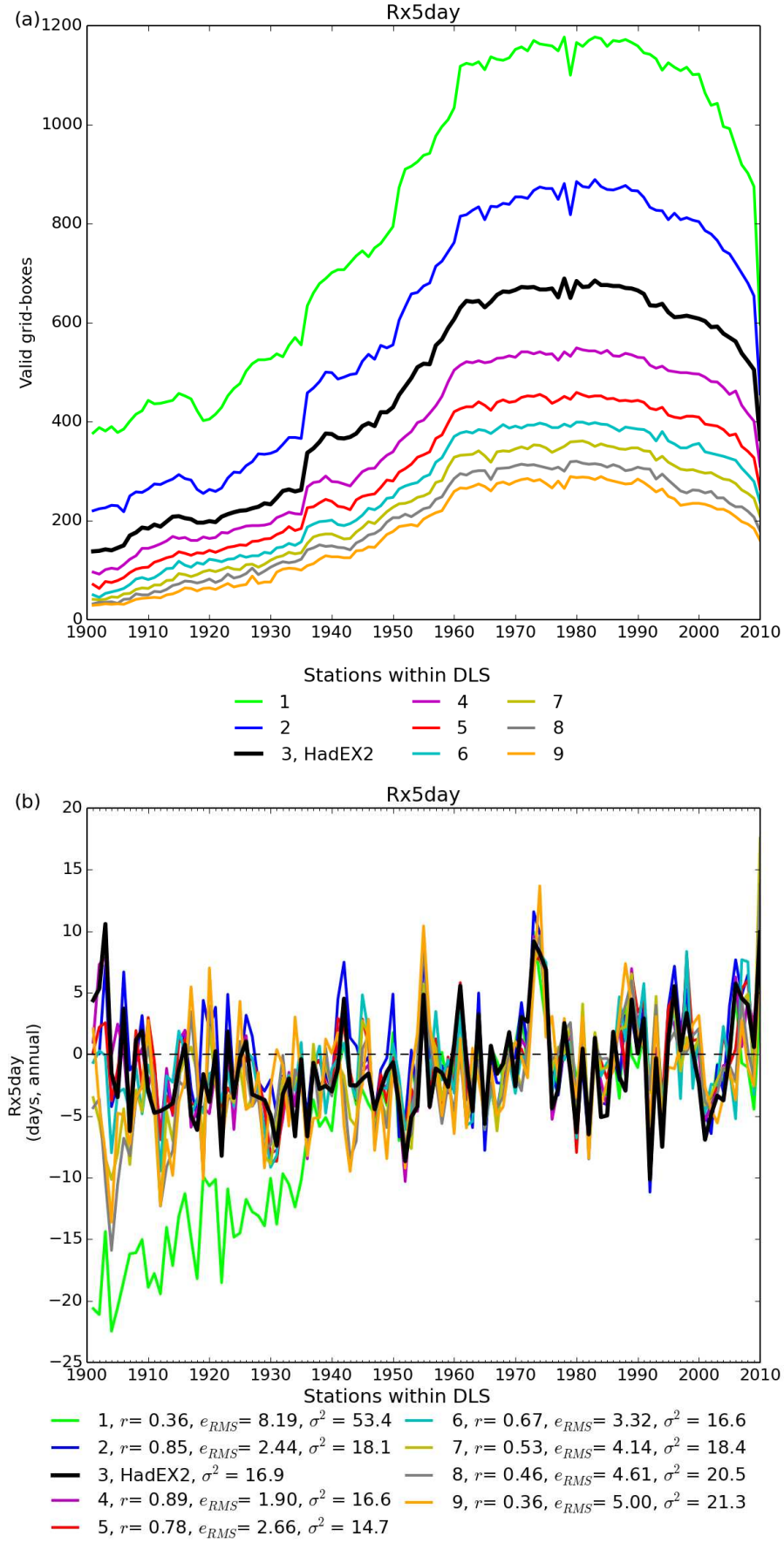
Figure 3: (a) : The number of non-missing grid boxes for Rx5day showing the different curves for left numbers of stations within a DLS of the grid box centre. Note that the global average only takes grid boxes which have 90 per cent completeness or more, whereas all grid boxes are shown in the coverage series. (b) : The time series for global average Rx5day.
