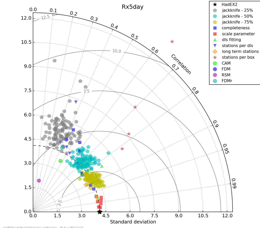
Figure 19: The Taylor Diagram for Rx5day calculated using the global average timeseries for each choice. Each of the different methodological choices are shown using a different symbol and colour as indicated in the legend.
