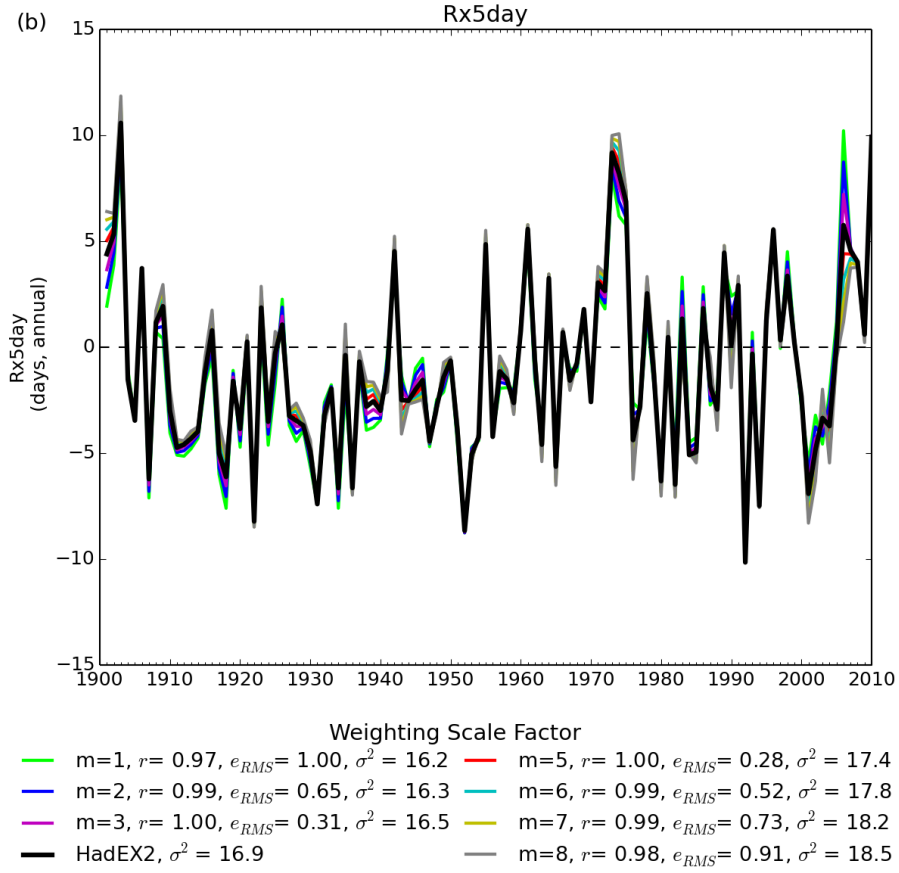
Figure 2: The time series for global average Rx5day showing the different curves for the different weighting values (colours are indicated below the plot). The figure also shows the correlation coefficient ( r ), variance ( \sigma^2 ) and root-mean-square error ( e_{RMS} ) between each series and HadEX2. All choices have been normalised over the 1961-1990 period.
