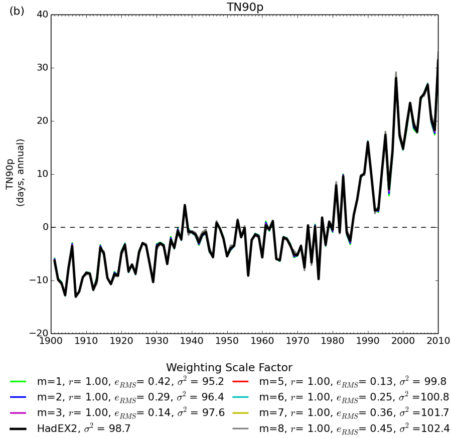
Figure 2: The time series for global average TN90p showing the different curves for the different weighting values (colours are indicated below the plot). The figure also shows the correlation coefficient ( r ), variance ( \sigma^2 ) and root-mean-square error ( e_{RMS} ) between each series and HadEX2. All choices have been normalised over the 1961-1990 period.
