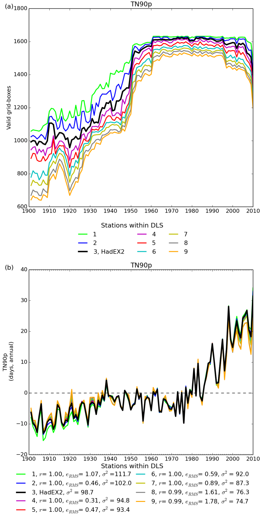
Figure 3: (a) : The number of non-missing grid boxes for TN90p showing the different curves for left numbers of stations within a DLS of the grid box centre. Note that the global average only takes grid boxes which have 90 per cent completeness or more, whereas all grid boxes are shown in the coverage series. (b) : The time series for global average TN90p.
