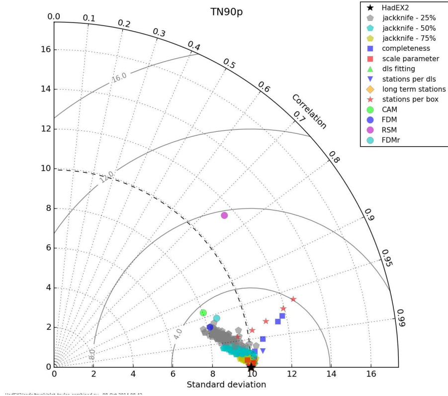
Figure 19: The Taylor Diagram for TN90p calculated using the global average timeseries for each choice. Each of the different methodological choices are shown using a different symbol and colour as indicated in the legend.
