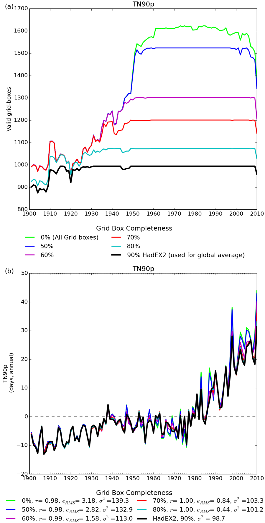
Figure 1: (a) The coverage, showing the different curves for different completeness requirements, for TN90p. The total coverage is shown the curve in light green, whereas the coverage used when calculating global averages is in black, with a range of other completeness percentages shown in between. (b) : The time series for global average of TN90p. Also shown are the comparison of other completenesses to that used in HadEX2 (90 %) using the correlation coefficient, r , the root mean square error e_{ems} and the variance, \sigma^2 .
