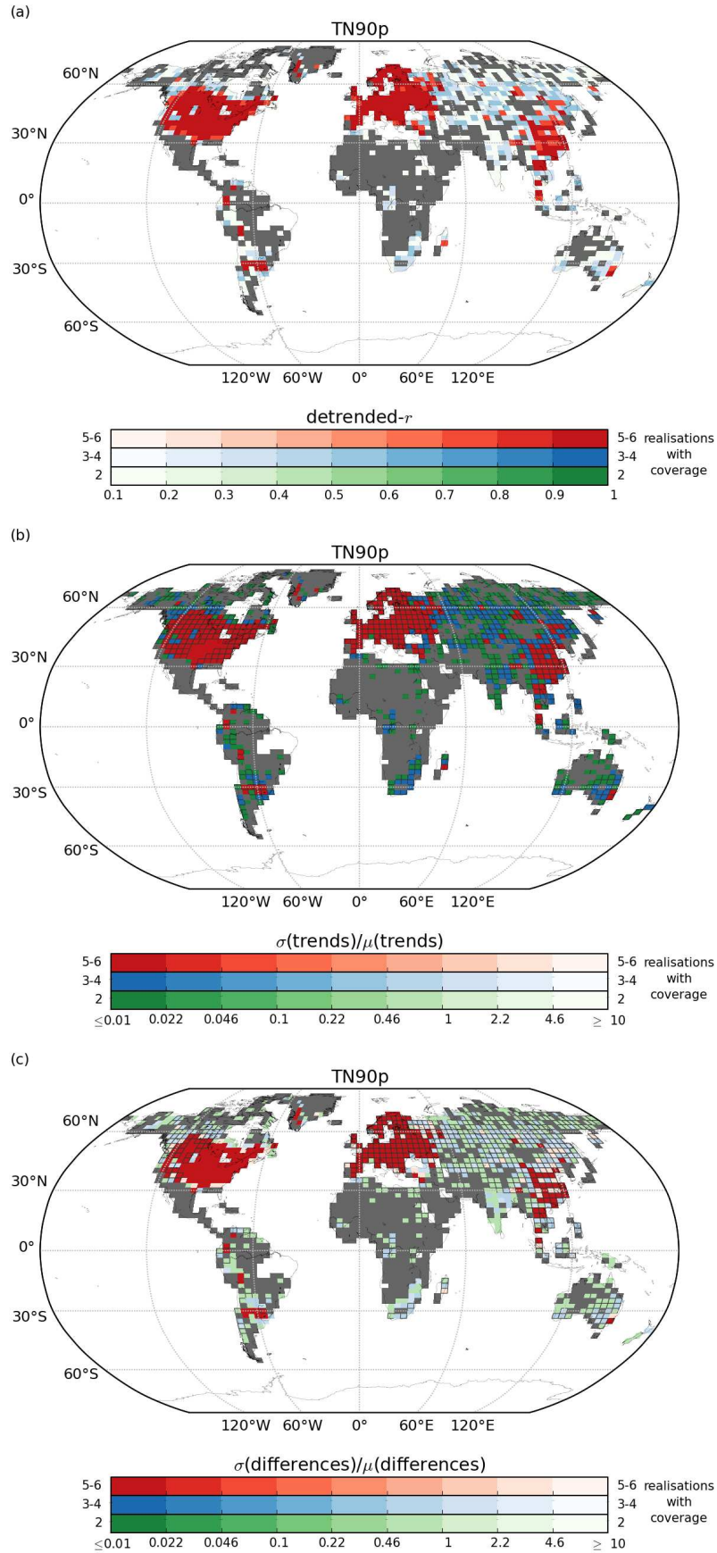
Figure 6: As for Fig. 4 but for TN90p restricted by the number of stations within a grid box. Grey grid boxes are those where only one of the 6 possible stations per grid box choices results in a value, green when 2, blue when 3-4 and red when 5-6 of the possible choices result in a value. Note that the HadEX2 method does not require any stations to be present within a grid box for a value to be calculated. In (b) and (c), boxes which have been outlined are ones where the trend was significant in the HadEX2 version. For details on the calculation method, see text.
