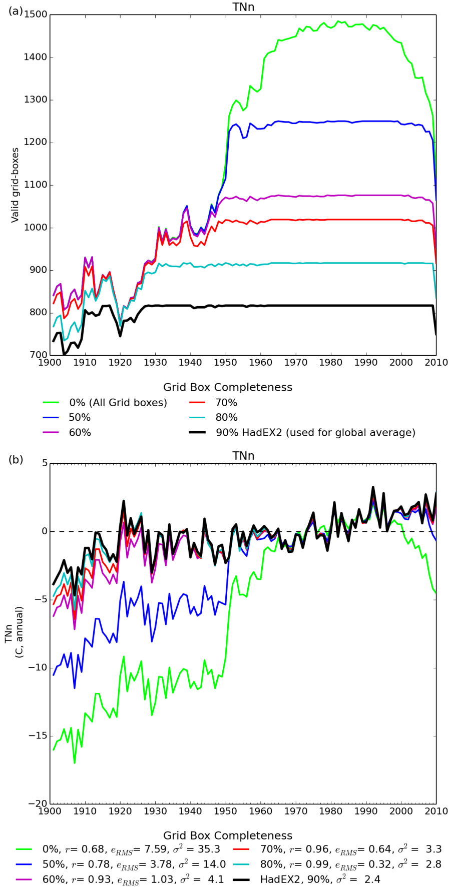
Figure 1: (a) The coverage, showing the different curves for different completeness requirements, for TNn. The total coverage is shown the curve in light green, whereas the coverage used when calculating global averages is in black, with a range of other completeness percentages shown in between. (b) : The time series for global average of TNn. Also shown are the comparison of other completenesses to that used in HadEX2 (90 %) using the correlation coefficient, r , the root mean square error e_{rms} and the variance, \sigma^2 .
