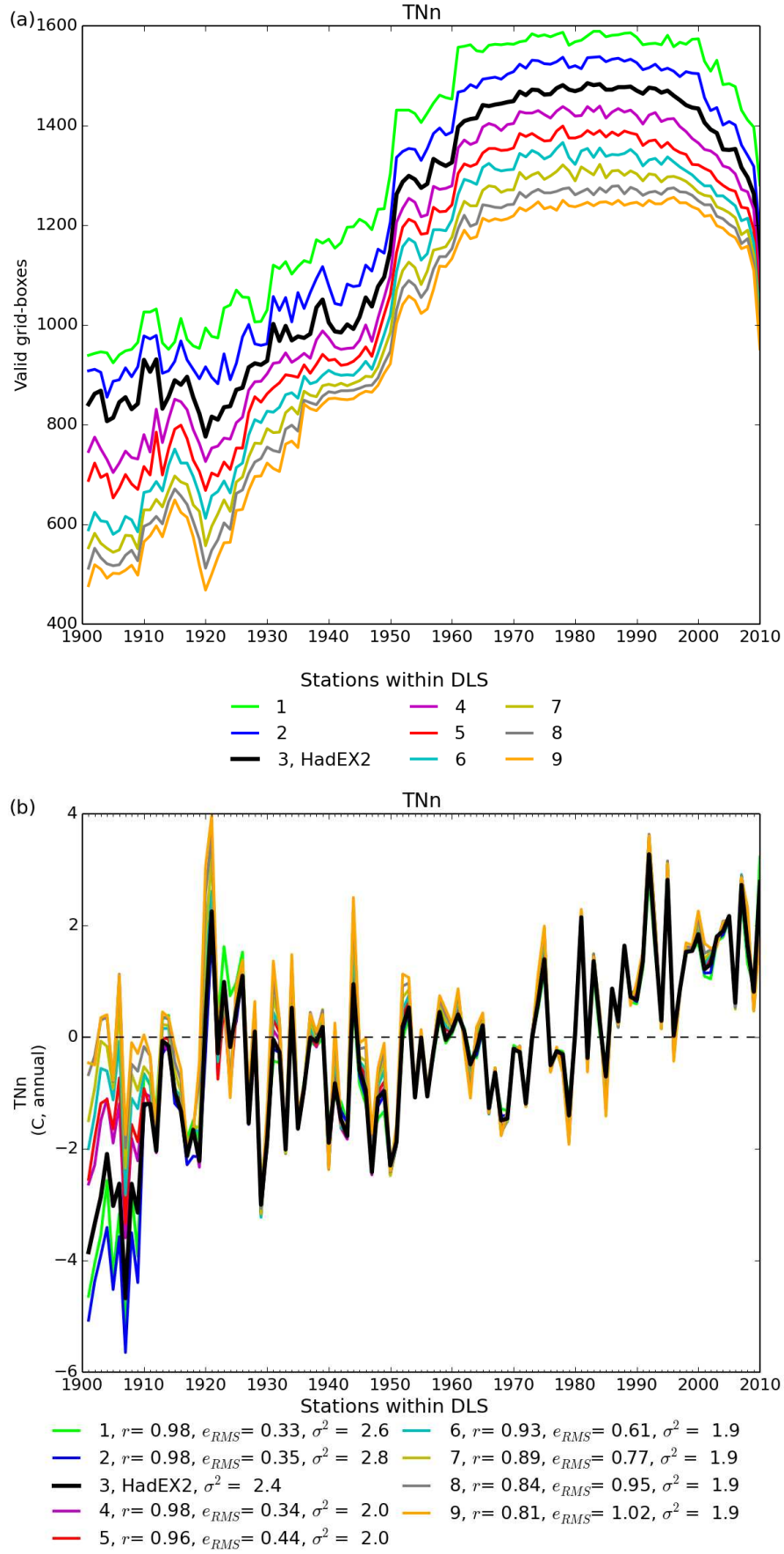
Figure 3: (a) : The number of non-missing grid boxes for T Nn showing the different curves for left numbers of stations within a DLS of the grid box centre. Note that the global average only takes grid boxes which have 90 per cent completeness or more, whereas all grid boxes are shown in the coverage series. (b) : The time series for global average T Nn .
