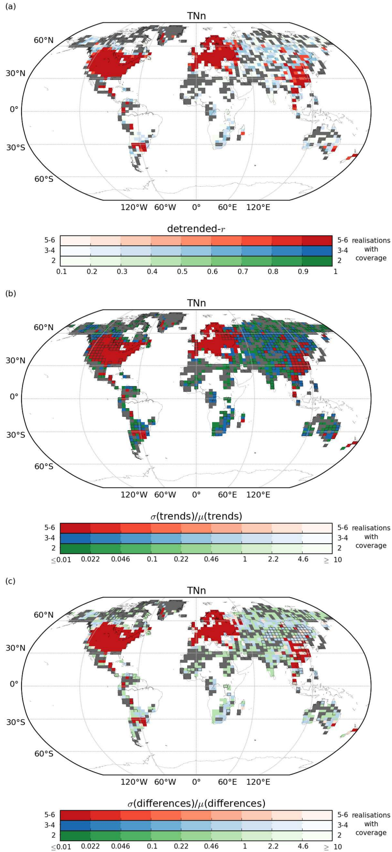
Figure 6: As for Fig. 4 but for TNn restricted by the number of stations within a grid box. Grey grid boxes are those where only one of the 6 possible stations per grid box choices results in a value, green when 2, blue when 3-4 and red when 5-6 of the possible choices result in a value. Note that the HadEX2 method does not require any stations to be present within a grid box for a value to be calculated. In (b) and (c), boxes which have been outlined are ones where the trend was significant in the HadEX2 version. For details on the calculation method, see text.
