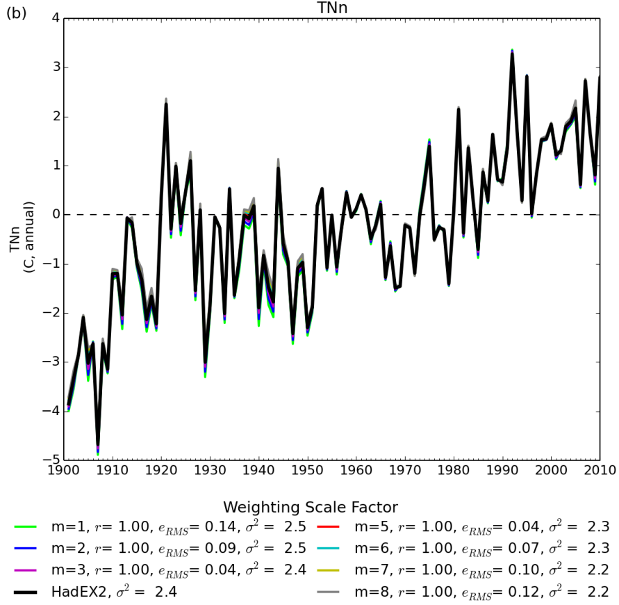
Figure 2: The time series for global average TNn showing the different curves for the different weighting values (colours are indicated below the plot). The figure also shows the correlation coefficient ( r ), variance ( \sigma^2 ) and root-mean-square error ( e_{RMS} ) between each series and HadEX2. All choices have been normalised over the 1961-1990 period.
