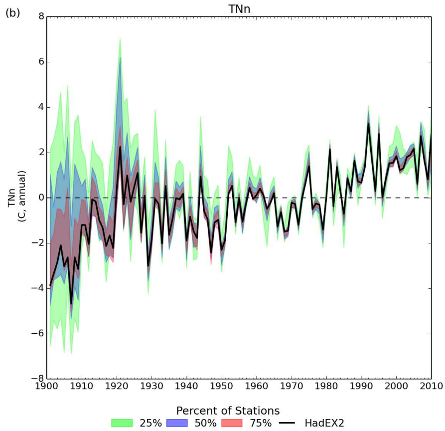
Figure 16: (a) : The number of non-missing grid boxes and (b) : the time series for the global average of TNn for the sub-sampling runs. Each colour shows the maximum range of the time series for each of the three sets of runs, 25% of stations in green, 50% in blue and 75% in purple respectively. Note that the global average only takes grid boxes which have 90 per cent completeness or more, whereas all grid boxes are shown in the coverage series.
