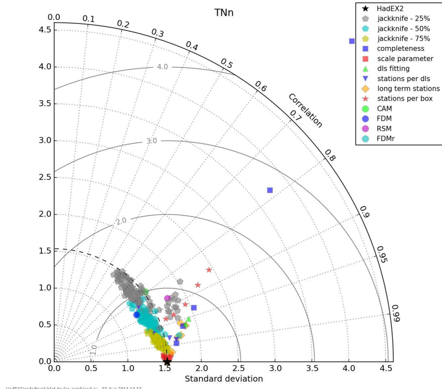
Figure 19: The Taylor Diagram for TNn calculated using the global average timeseries for each choice. Each of the different methodological choices are shown using a different symbol and colour as indicated in the legend.
