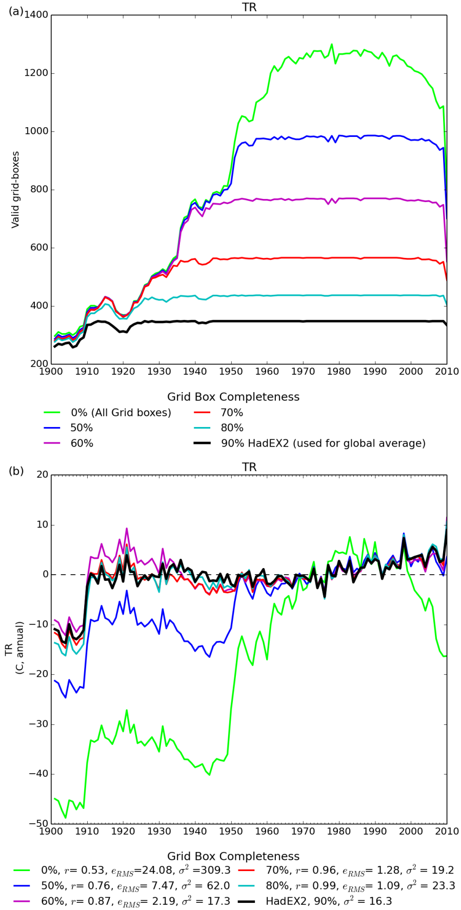
Figure 1: (a) The coverage, showing the different curves for different completeness requirements, for TR. The total coverage is shown the curve in light green, whereas the coverage used when calculating global averages is in black, with a range of other completeness percentages shown in between. (b) : The time series for global average of TR. Also shown are the comparison of other completenesses to that used in HadEX2 (90 %) using the correlation coefficient, r , the root mean square error e_{ems} and the variance, \sigma^2 .
