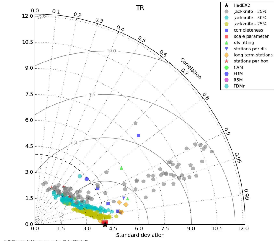
Figure 19: The Taylor Diagram for TR calculated using the global average timeseries for each choice. Each of the different methodological choices are shown using a different symbol and colour as indicated in the legend.
