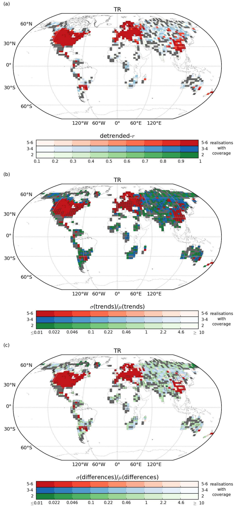
Figure 6: As for Fig. 4 but for TR restricted by the number of stations within a grid box. Grey grid boxes are those where only one of the 6 possible stations per grid box choices results in a value, green when 2, blue when 3-4 and red when 5-6 of the possible choices result in a value. Note that the HadEX2 method does not require any stations to be present within a grid box for a value to be calculated. In (b) and (c), boxes which have been outlined are ones where the trend was significant in the HadEX2 version. For details on the calculation method, see text.
