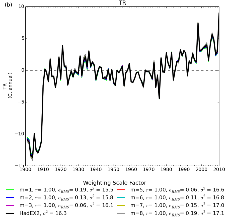
Figure 2: The time series for global average TR showing the different curves for the different weighting values (colours are indicated below the plot). The figure also shows the correlation coefficient ( r ), variance ( \sigma^2 ) and root-mean-square error ( e_{RMS} ) between each series and HadEX2. All choices have been normalised over the 1961-1990 period.
