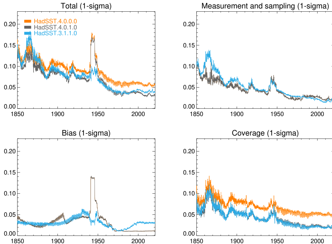
Figure 3: Uncertainty components from HadSST.4.0.0.0 (orange), 4.0.1.0 (grey) and 3.1.1.0 (blue) including total uncertainty (top left), measurement and sampling uncertainty (top right), bias uncertainty (bottom left) and coverage uncertainty (bottom right). The HadSST.4.0.0.0 coverage uncertainty is erroneously large. Note that the measurement and sampling uncertainties and the bias uncertainties are identical in versions 4.0.1.0 and 4.0.0.0 except for the final three months of 2020 so the grey line overlays the orange line almost completely, rendering it all but invisible.
